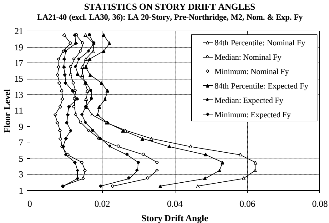
Figure 8.16 Sensitivity of Story Drift Angle Demands to Strength of Material, LA 20-story Structure; 2/50 Set of Ground Motions
