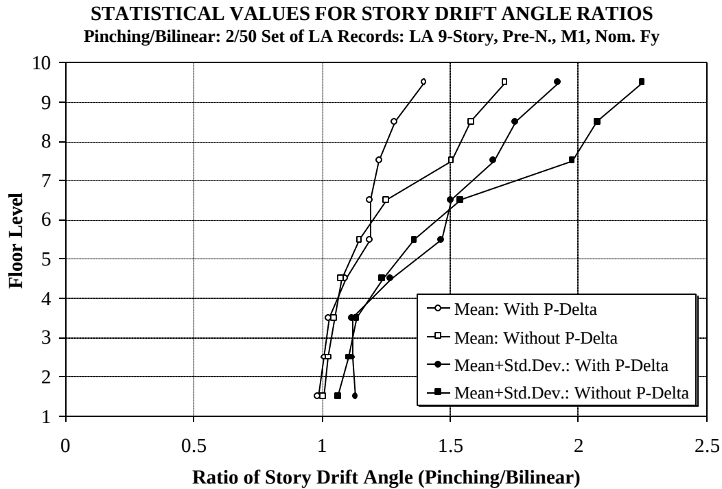
Figure 8.7 Story Drift Angle Ratios (Pinching Model/Bilinear Model) with and without P-delta Effect, LA 9-story Structure; 2/50 Set of Ground Motions
