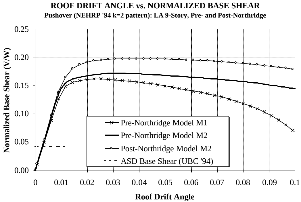
Figure 5.2 Global Pushover Curves for LA 9-story Structures
