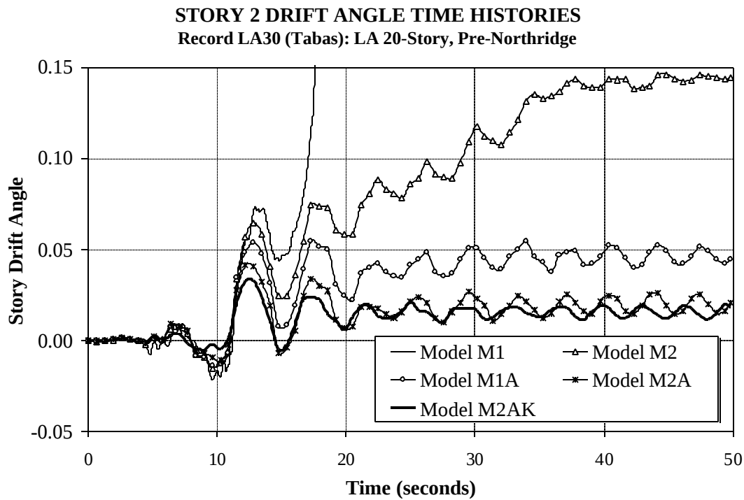
Figure 4.16a Time Histories of Story 2 Drift Angle for Various Models of LA 20-story Structure; LA30 (Tabas) Ground Motion
