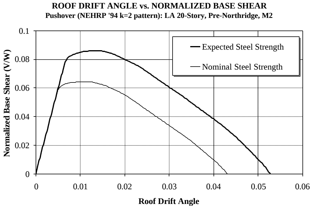
Figure 8.15 Sensitivity of Global Pushover Curves to Strength of Material, LA 20-story Structure; Pushover Analysis
