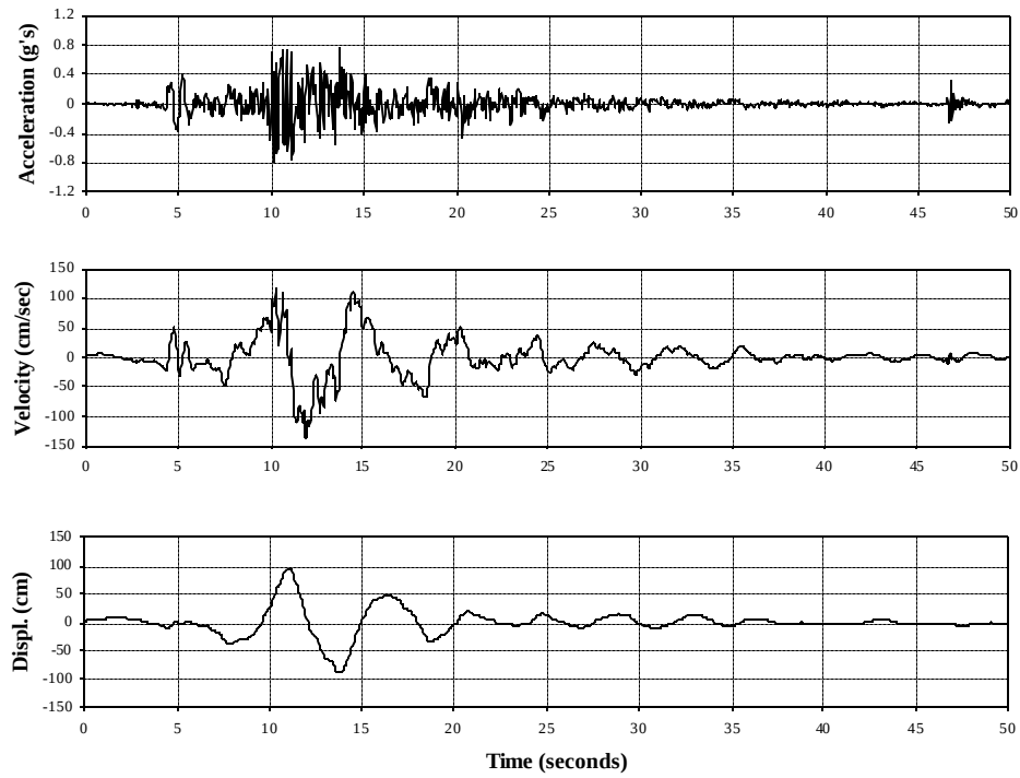
Figure 4.9 Time History of Record LA30 (Tabas) Used for P-delta Study of LA 20-story Structure
