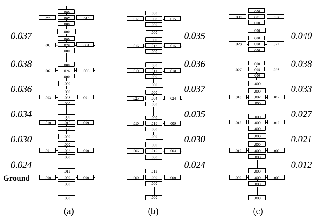
Figure 6.6 Story and Element Deformation Demands at 3% Roof Drift Angle, for Seattle 9-story Str. (a) Pre-N., (b) Cover-Plated Post-N., (c) RBS; Pushover Analysis
