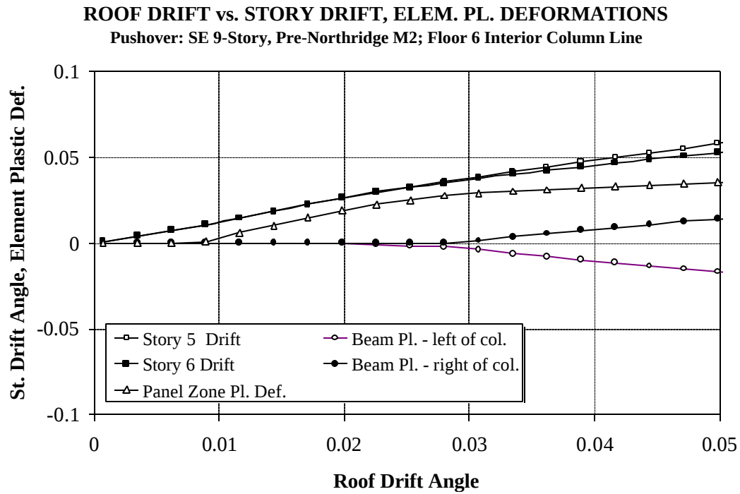
Figure 6.7 Variation of Story and Element Deformation Demands with Increasing Roof Drift Angle for Seattle 9-story Pre-N. Structure; Pushover Analysis
