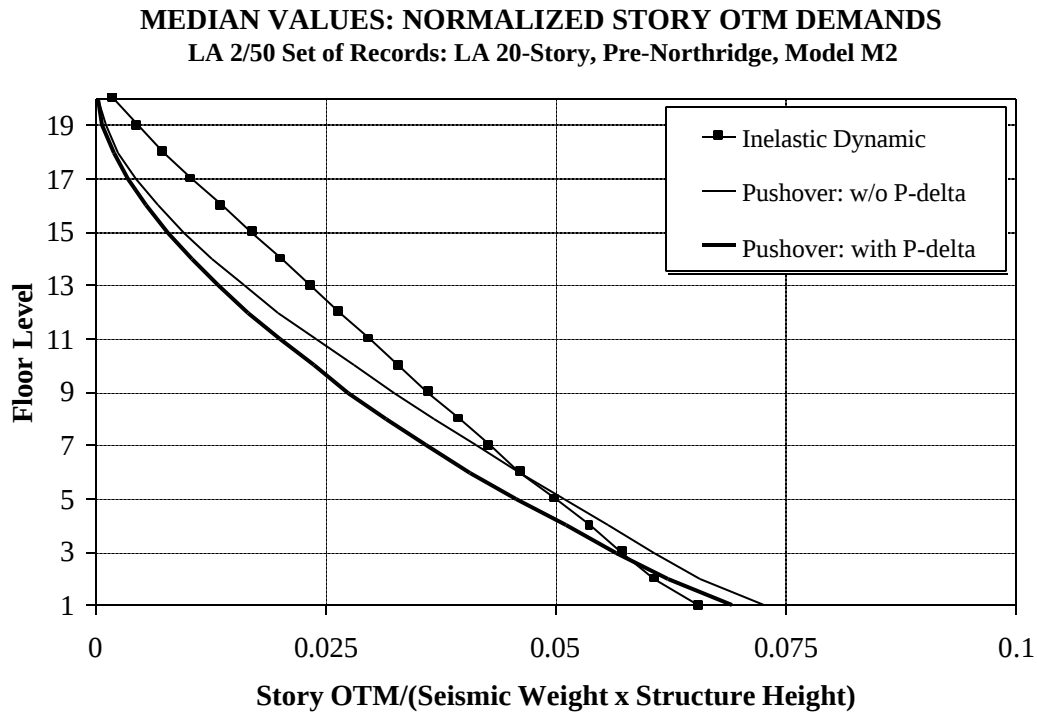
Figure 5.58. Median Story OTM Demands Under 2/50 Sets of Ground Motions, Compared to Demands From Pushover Analysis, for Inelastic LA 20-story Structure
