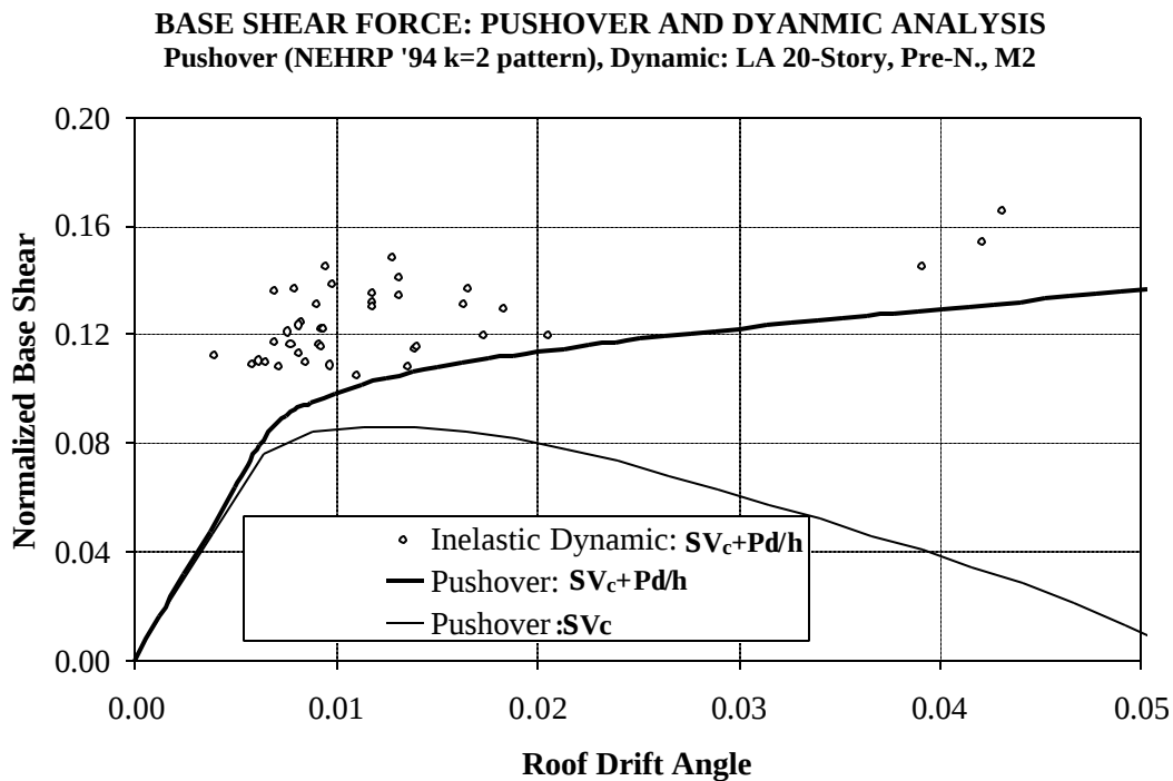
Figure 5.55 Median Values of Base and Story Shear Forces for LA 20-story Structure; 2/50 Set of Ground Motions, and from Pushover Analysis
