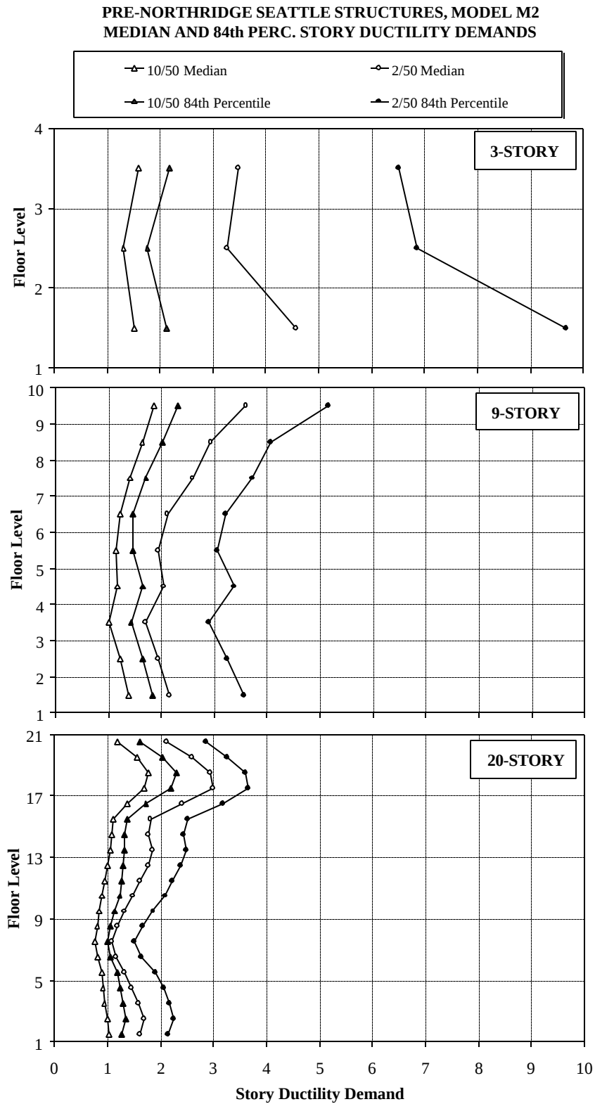
Figure 5.35 Median and 84 th Percentile Story Ductility Demands for Seattle Structures, Model M2; 10/50 and 2/50 Sets of Ground Motions
