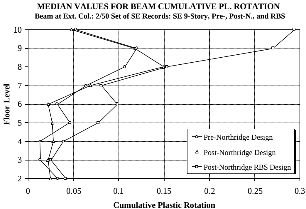
Figure 6.36 Statistical Values for Exterior Beam End Cumulative Plastic Rotation Demands, SE 9-story Structure, Different Designs; 2/50 Set of Ground Motions
