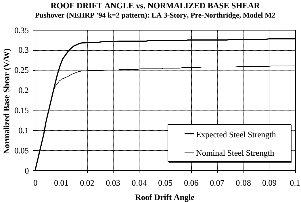
Figure 8.13 Sensitivity of Global Pushover Curves to Strength of Material, LA 3-story Structure; Pushover Analysis
