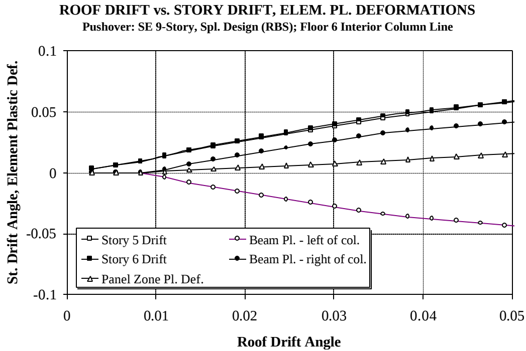
Figure 6.9 Variation of Story and Element Deformation Demands with Increasing Roof Drift Angle for Seattle 9-story RBS Design; Pushover Analysis
