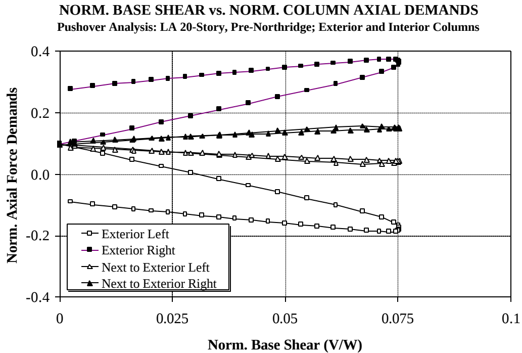
Figure 6.30 Variation of Story 1 Column Force Demands with Base Shear Demand, LA 20-story Structure; Pushover Analysis
