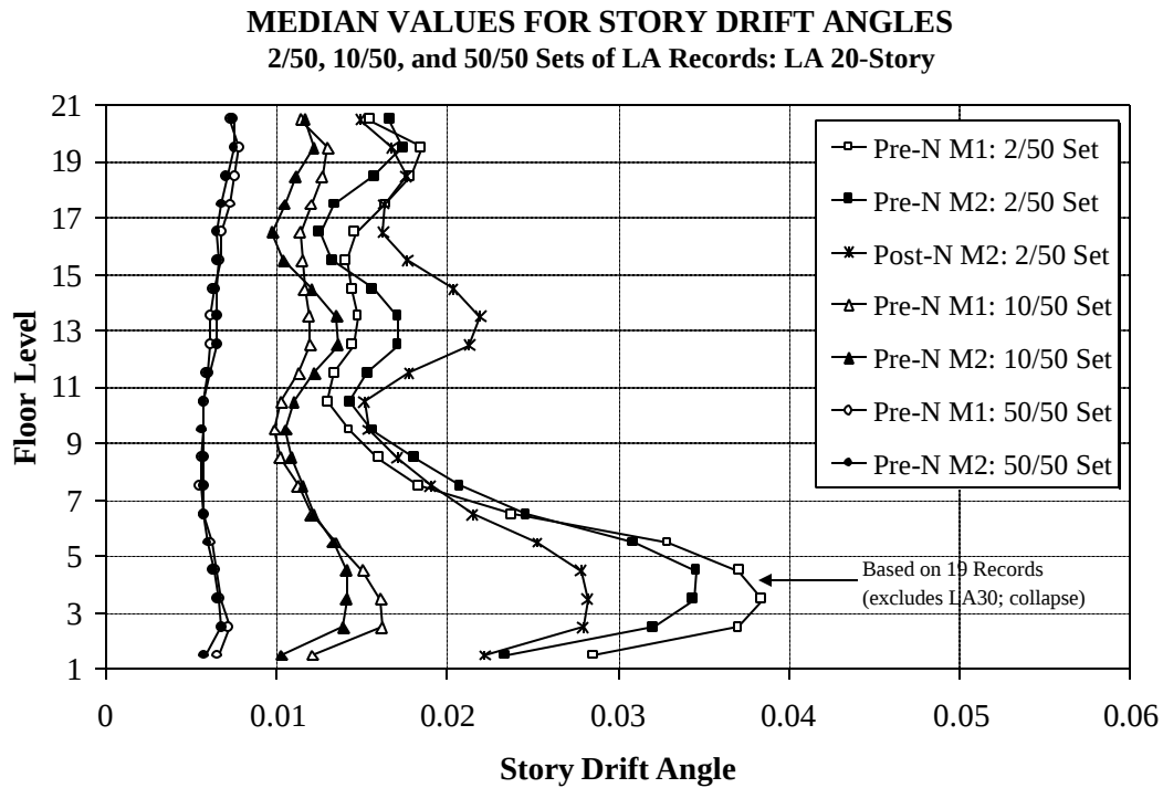
Figure 5.21 Median Values of Story Drift Angle Demands for LA 20-story Structures; 50/50, 10/50, and 2/50 Sets of Ground Motions
