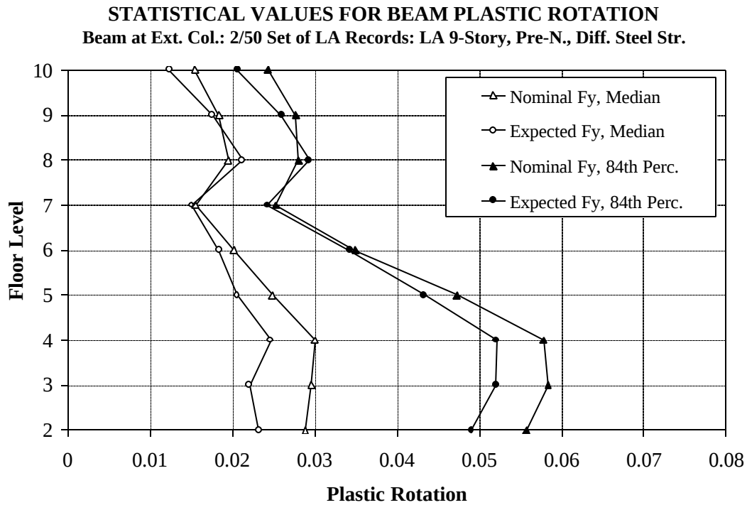
Figure 6.13 Beam (@ Exterior Col.) Plastic Rotation Demands for LA 9-story Structure with Expected and Nominal Strength Properties; 2/50 Set of Ground Motions
