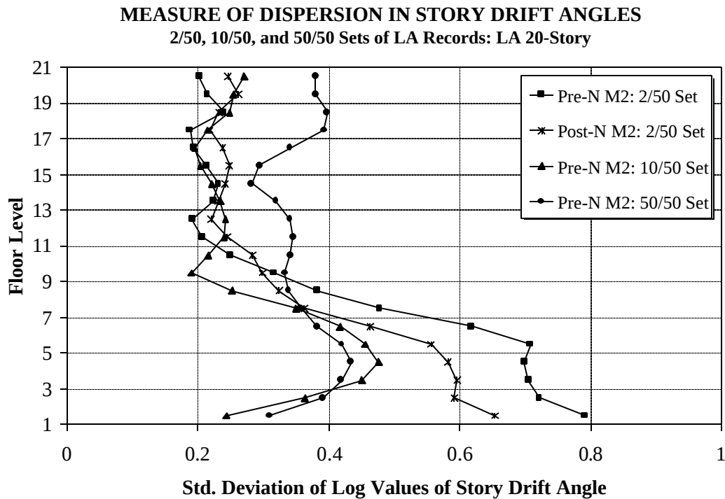
Figure 5.22 Measure of Dispersion of Story Drift Angle Demands for LA 20-story Structures; 50/50, 10/50, and 2/50 Sets of Ground Motions
