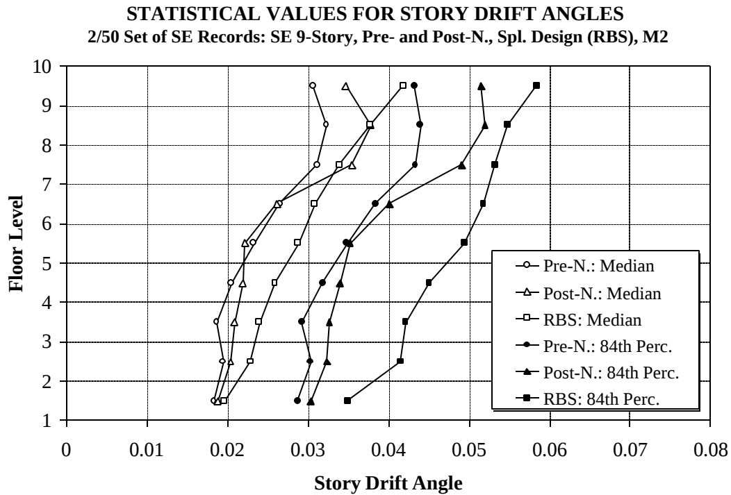
Figure 6.17 Story Drift Angle Demands for Seattle 9-story Pre-N., Cover-Plated Post-N., and RBS Design; 2/50 Set of Ground Motions
