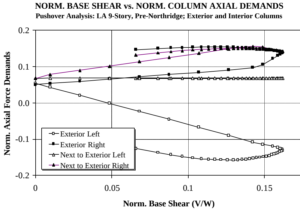
Figure 6.29 Variation of Story 1 Column Force Demands with Base Shear Demand, LA 9-story Structure; Pushover Analysis
