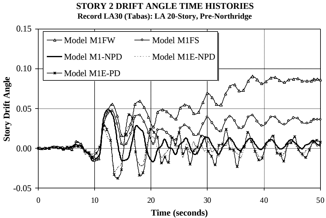
Figure 4.16b Time Histories of Story 2 Drift Angle for Various Models of LA 20-story Structure; LA30 (Tabas) Ground Motion
