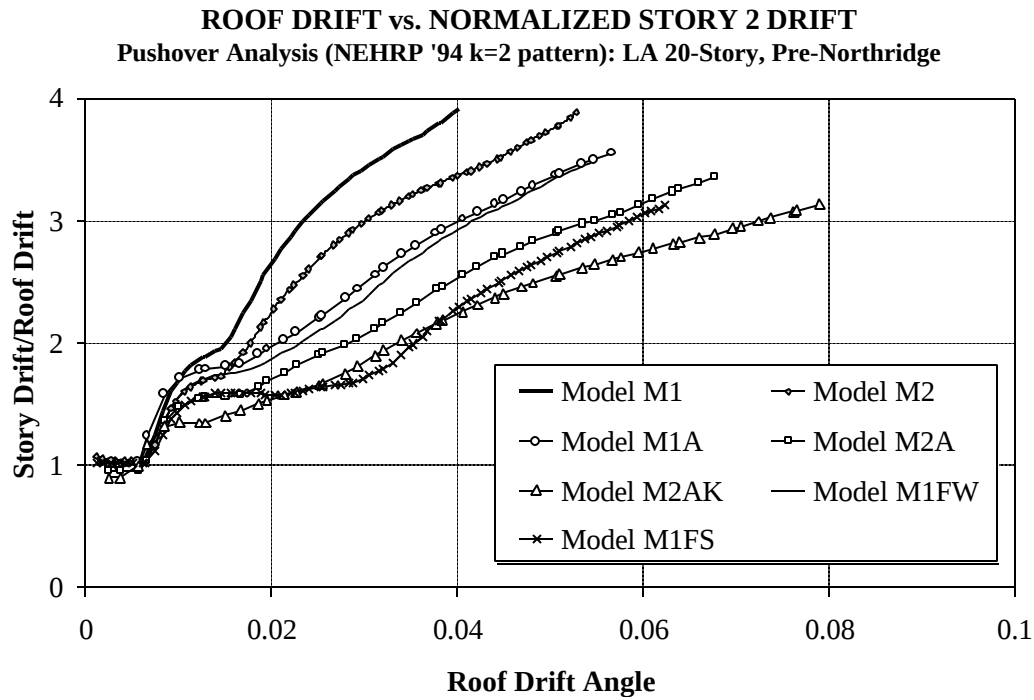
Figure 4.15 Ratios of Story 2 Drift Angle to Roof Drift Angle, Plotted Against Roof Drift Angle for Various Models of LA 20-story Structure
