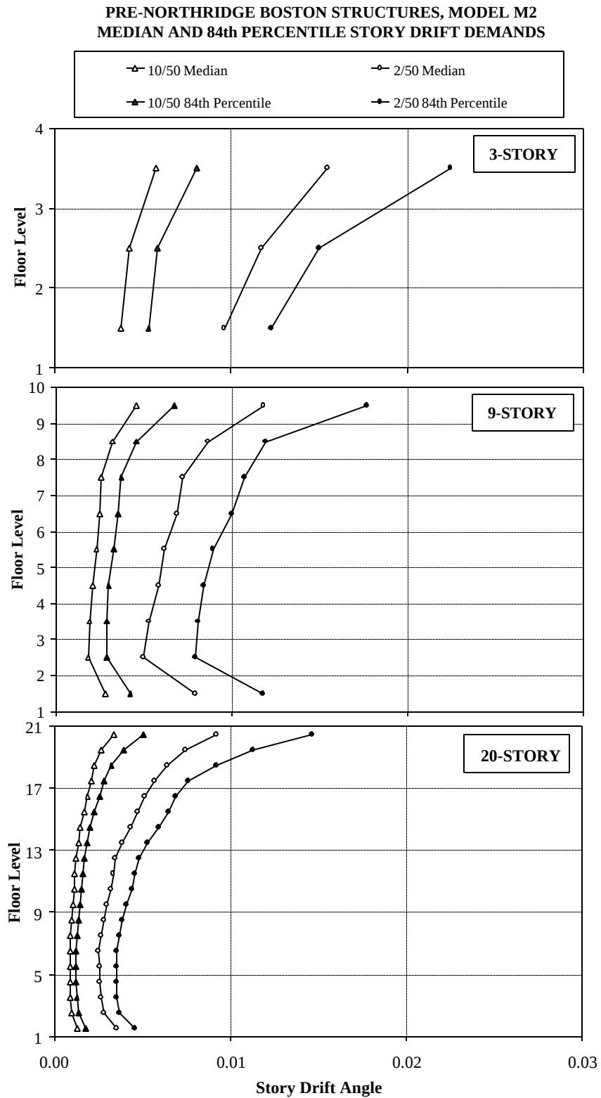
Figure 5.33 Median and 84 th Percentile Story Drift Angle Demands for Boston Structures, Model M2; 10/50 and 2/50 Sets of Ground Motions
