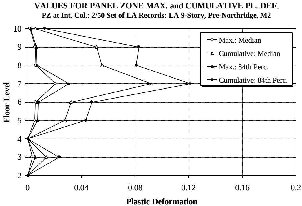
Figure 6.35 Statistical Values for Interior Panel Zone Maximum and Cumulative Plastic Deformation Demands, LA 9-story Structure; 2/50 Set of Ground Motions
