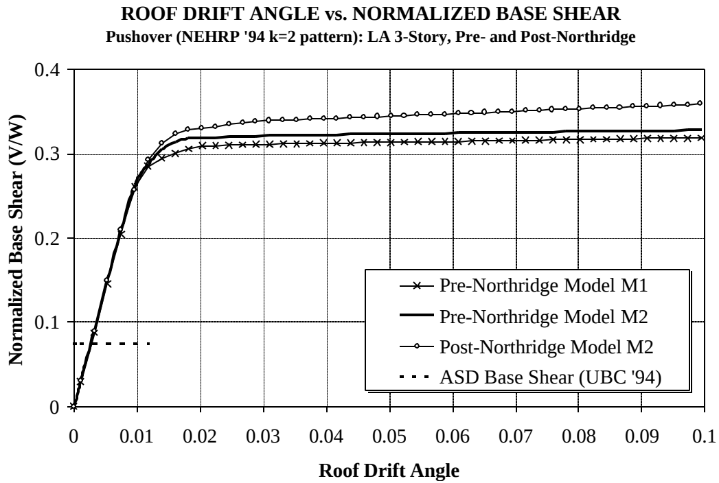
Figure 5.1 Global Pushover Curves for LA 3-story Structures
