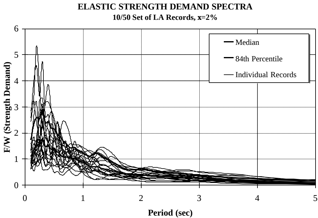
Figure A.3 Elastic Strength Demand (Acceleration) Spectra, 10/50 Set of LA Ground Motions
