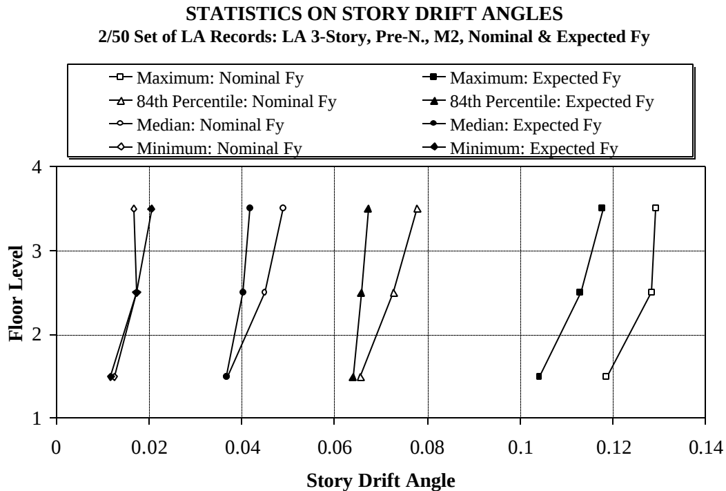
Figure 8.14 Sensitivity of Story Drift Angle Demands to Strength of Material, LA 3-story Structure; 2/50 Set of Ground Motions
