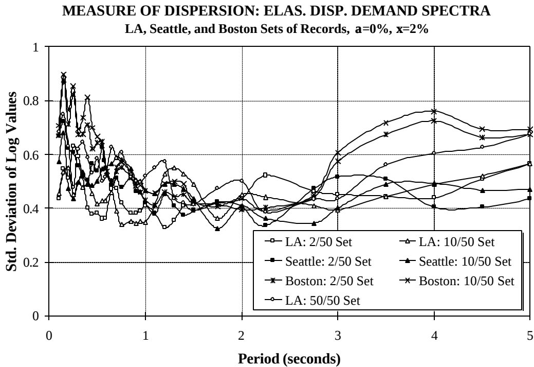
Figure 5.18 Measure of Dispersion of Elastic Spectral Displacement Demands for LA, Seattle, and Boston Sets of Ground Motions
