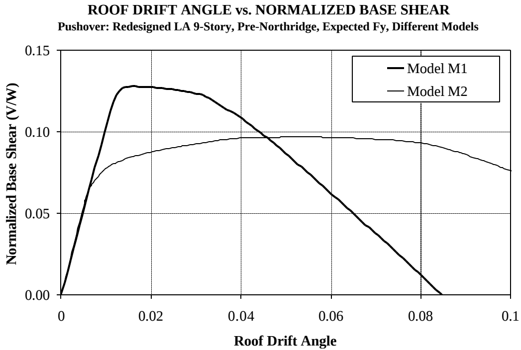
Figure 6.21 Global Pushover Curves for Redesigned LA 9-story Structure, for Different Analytical Models (M1 and M2)
