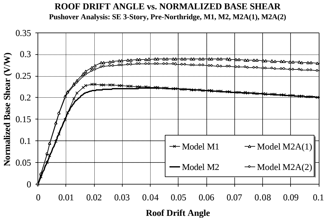
Figure 3.11 Global Pushover Curves for Seattle 3-story Structure, Different Models
