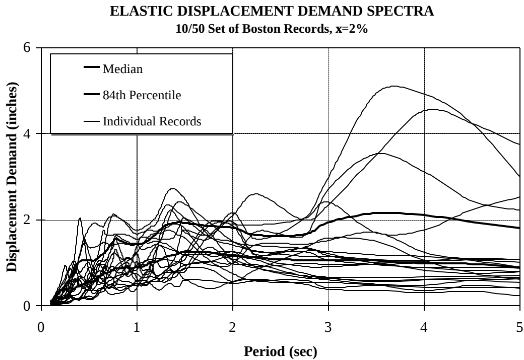
Figure A.12 Elastic Displacement Demand Spectra, 10/50 Set of Boston Ground Motions
