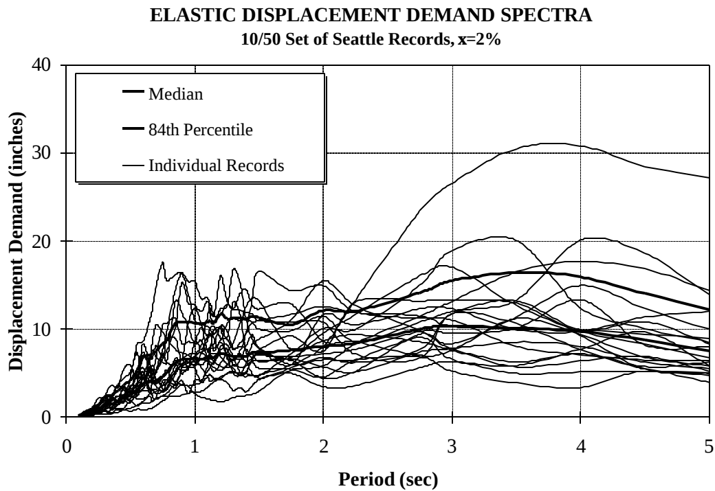
Figure A.8 Elastic Displacement Demand Spectra, 10/50 Set of Seattle Ground Motions
