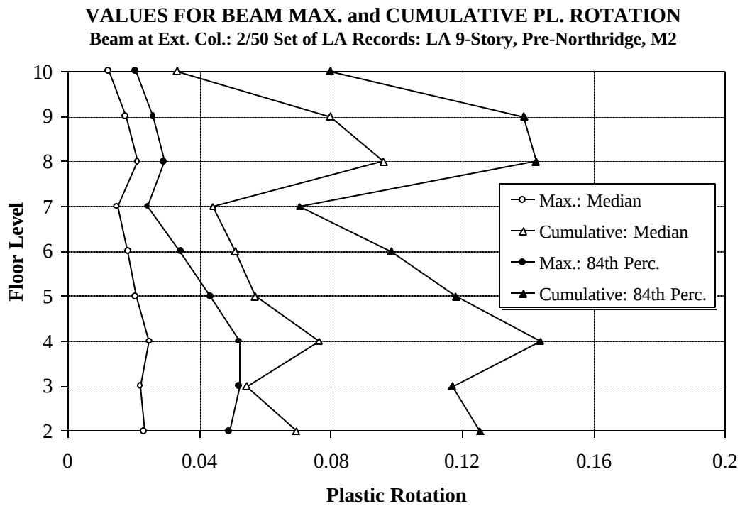
Figure 6.33 Statistical Values for Exterior Beam End Maximum and Cumulative Plastic Rotation Demands, LA 9-story Structure; 2/50 Set of Ground Motions
