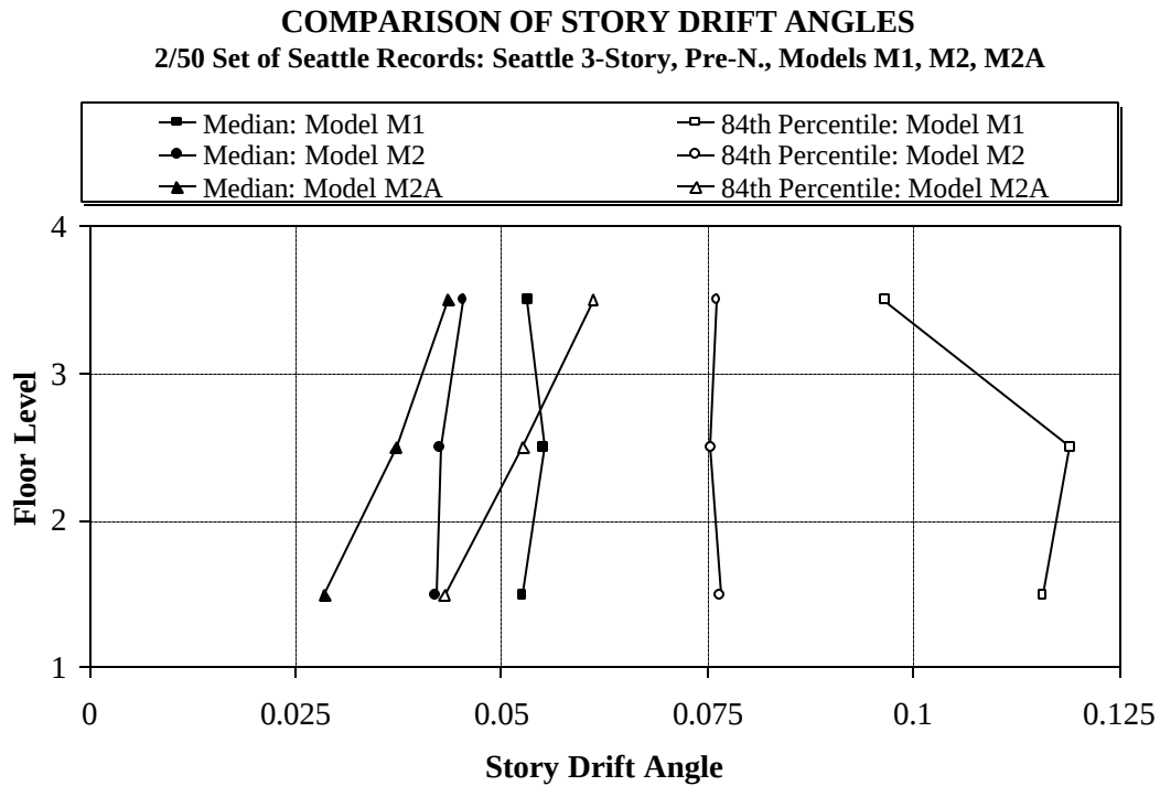
Figure 3.19 Median and 84 th Percentile Values of Story Drift Demands for Seattle 3-story Structure, Different models; 2/50 Set of Ground Motions
