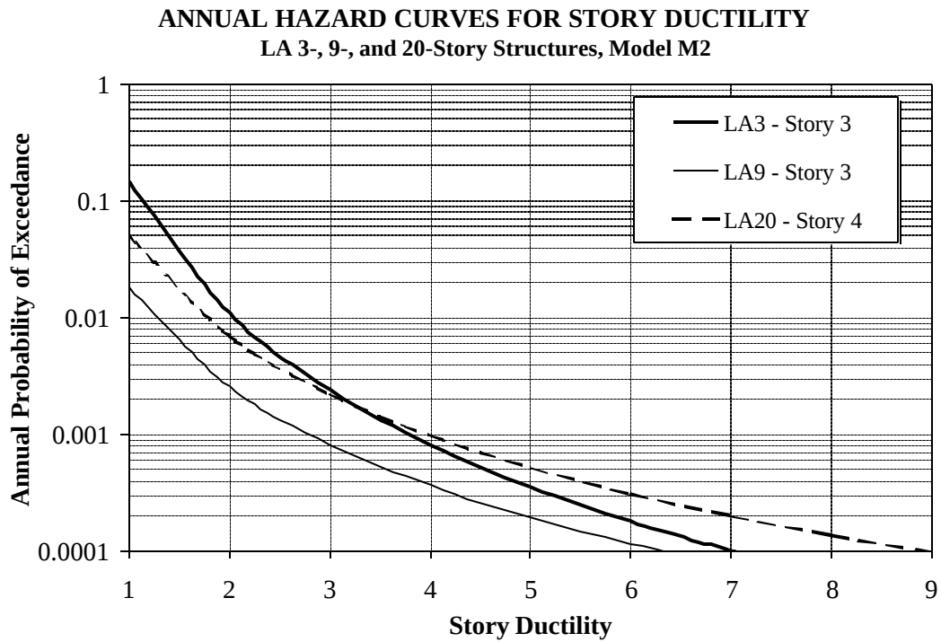
Figure 5.50 Annual Hazard Curves for Story Ductility Demand for LA 3-, 9-, and 20-story Structures
