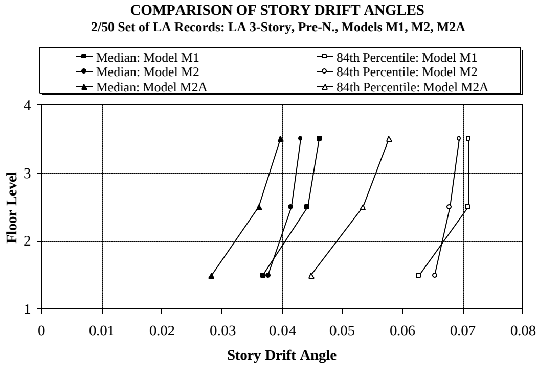
Figure 3.18 Median and 84 th Percentile Values of Story Drift Demands for LA 3-story Structure, Different models; 2/50 Set of Ground Motions
