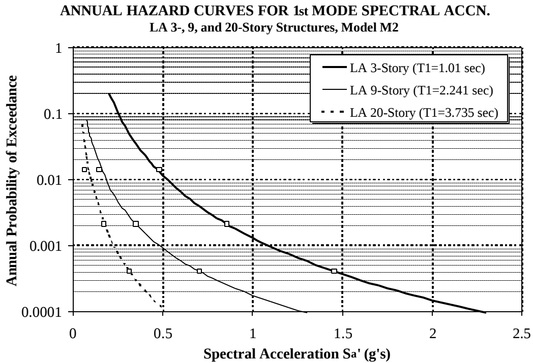
Figure 5.46 Annual Hazard Curves for 1 st Mode Spectral Acceleration for LA 3-, 9-, and 20-story Structures
