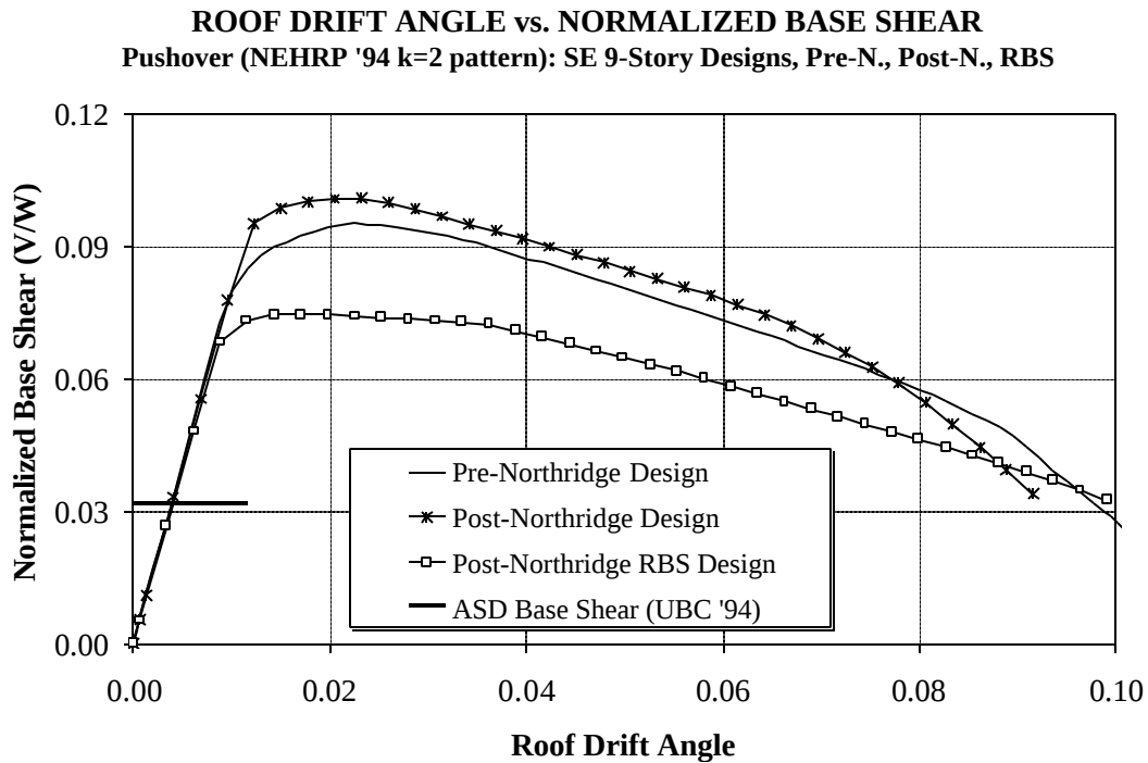
Figure 6.5 Global Pushover Curves for Seattle 9-story Structures, with Different Design Details
