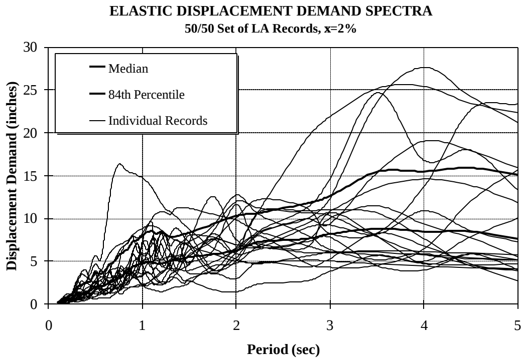
Figure A.2 Elastic Displacement Demand Spectra, 50/50 Set of LA Ground Motions
