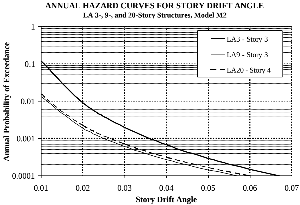
Figure 5.49 Annual Hazard Curves for Story Drift Angle Demand for LA 3-, 9-, and 20-story Structures
