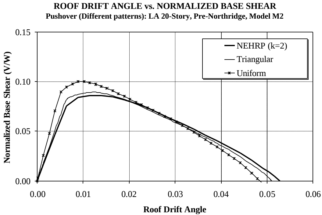
Figure 7.19 Effect of Load Pattern on Global (Roof) Pushover Response for LA 20-story Structure, Model M2
