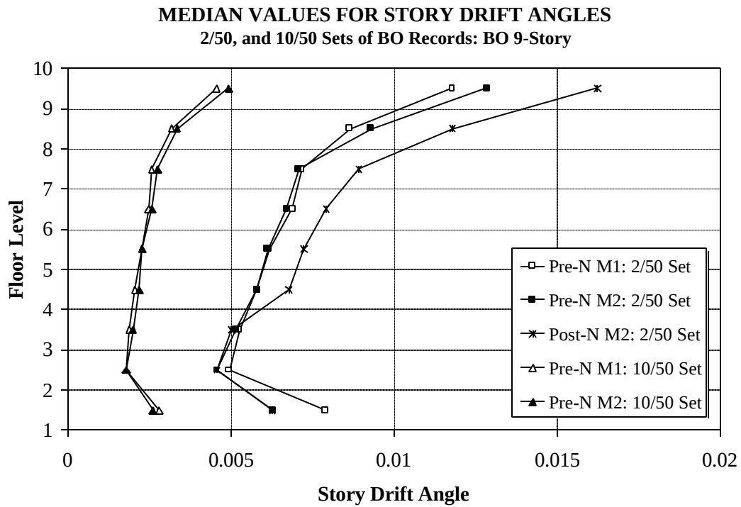
Figure 5.28 Median Values of Story Drift Angle Demands for Boston 9-story Structures; 10/50 and 2/50 Sets of Ground Motions
