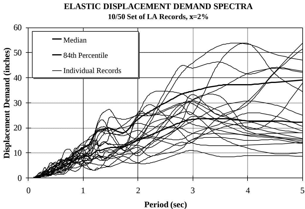
Figure A.4 Elastic Displacement Demand Spectra, 10/50 Set of LA Ground Motions
