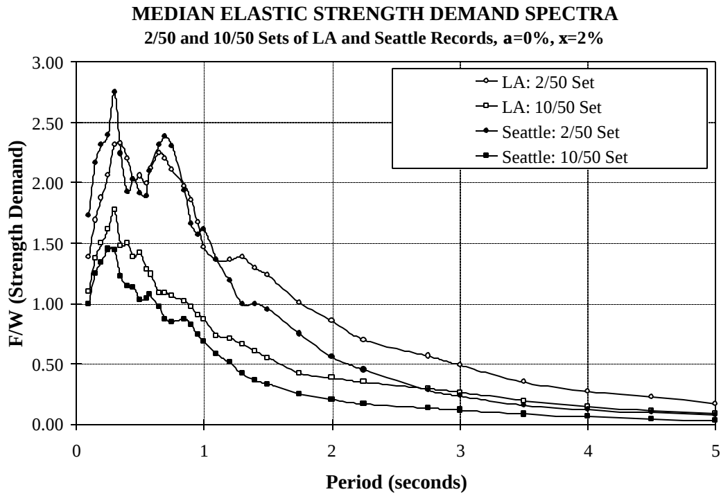
Figure 5.60 Comparison of Median Elastic Spectra for LA and Seattle 10/50 and 2/50 Sets of Ground Motions
