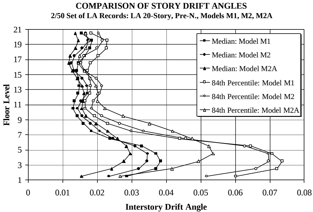
Figure 3.21 Median and 84 th Percentile Values of Story Drift Demands for LA 20-story Structure, Different Models; 2/50 Set of Ground Motions
