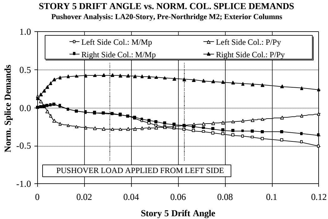
Figure 6.31 Variation of Normalized Force Demands for Exterior Column Splices in Story 5 with Increasing Story 5 Drift; LA 20-story; Pushover Analysis
