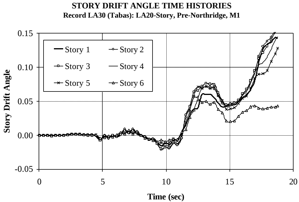
Figure 4.11 Story 1-6 Drift Angle Time Histories for Model M1 of LA 20-story Structure; LA30 (Tabas) Ground Motion
