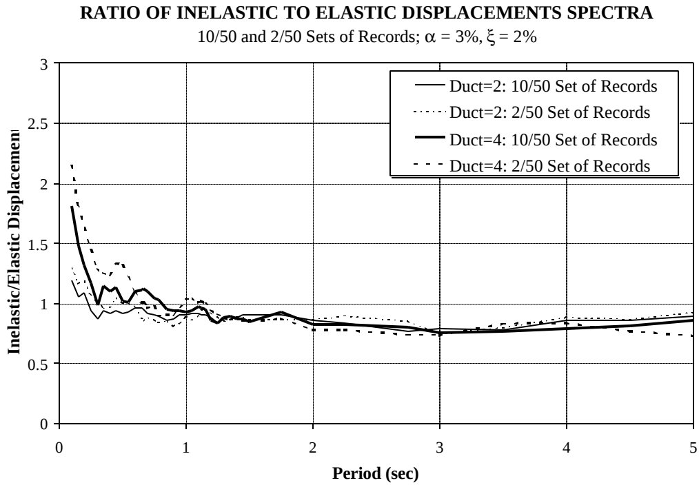
Figure 7.7 Median Values for Inelastic/Elastic Displacements for SDOF Systems, \alpha = 3\% , \xi = 2\% ; 10/50 and 2/50 Sets of LA Ground Motions
