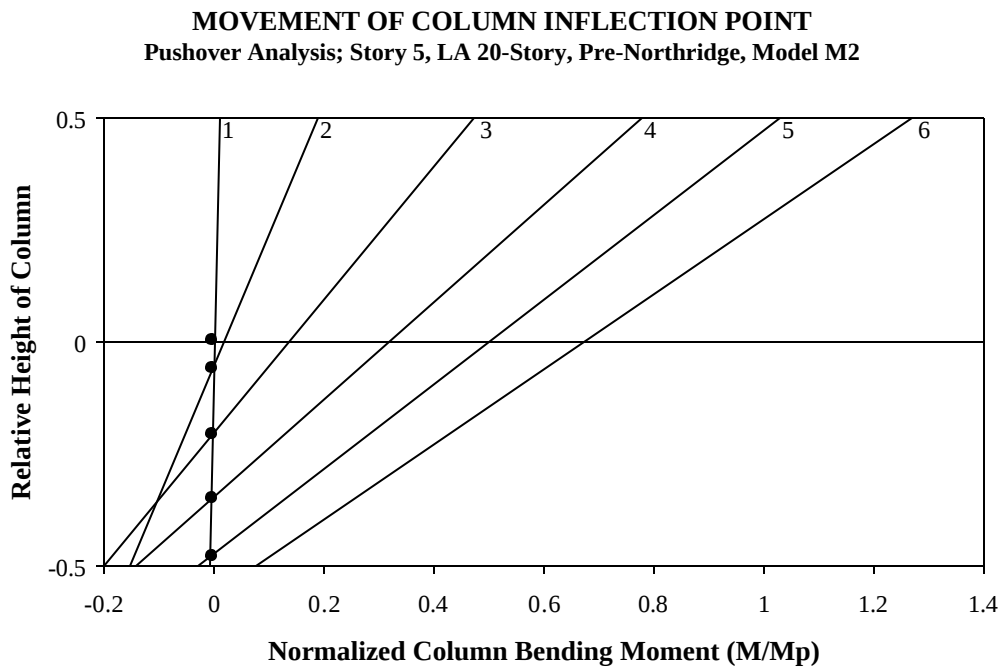
Figure 6.24 Movement of Column Inflection Point in Story 5 with Increasing Story Drift, LA 20-story; Pushover Analysis
