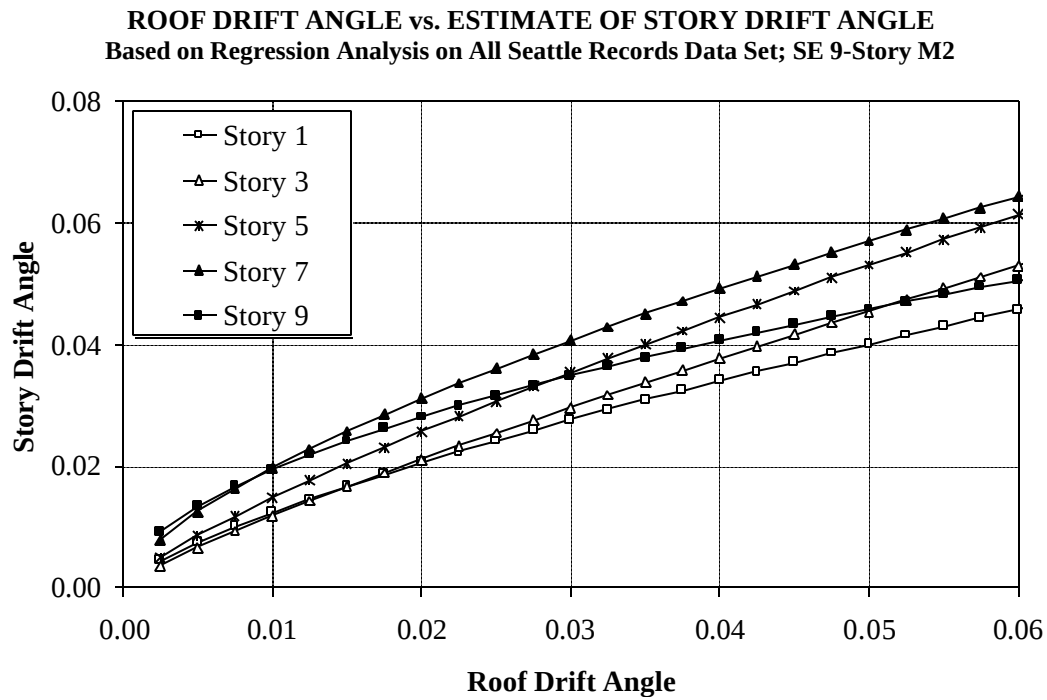
Figure 7.34 Relationship Between Story Drift Angles and Roof Drift Angle for SE 9-story Structure, Based on Regression Analysis; All Seattle Records
