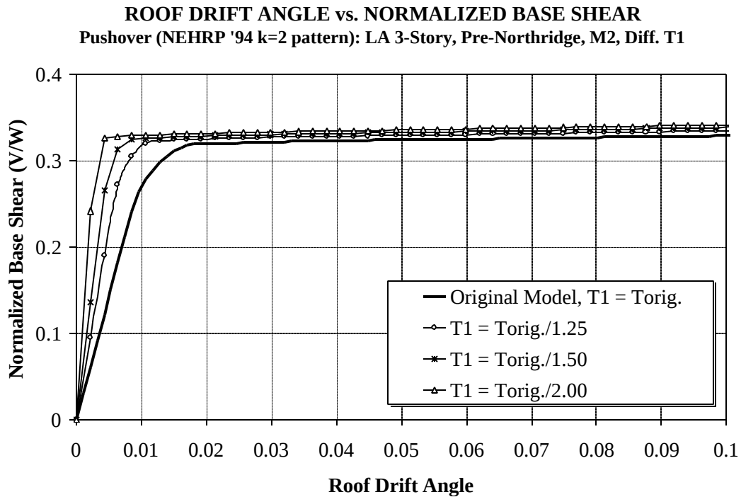
Figure 8.17 Sensitivity of Global Pushover Curves to Period of Structure, LA 3-story Structure; Pushover Analysis
