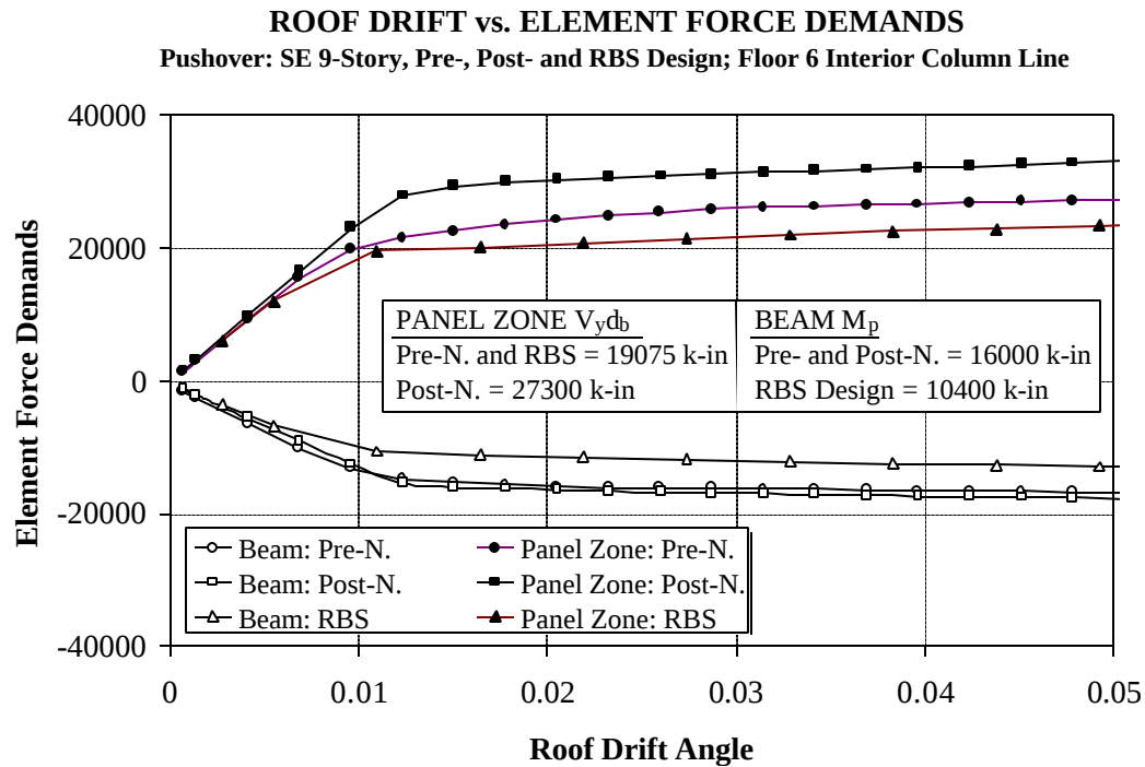
Figure 6.10 Variation of Element Force Demands with Increasing Roof Drift Angle for Seattle 9-story Pre-N., Cover-Plated Post-N., and RBS Design; Pushover Analysis
