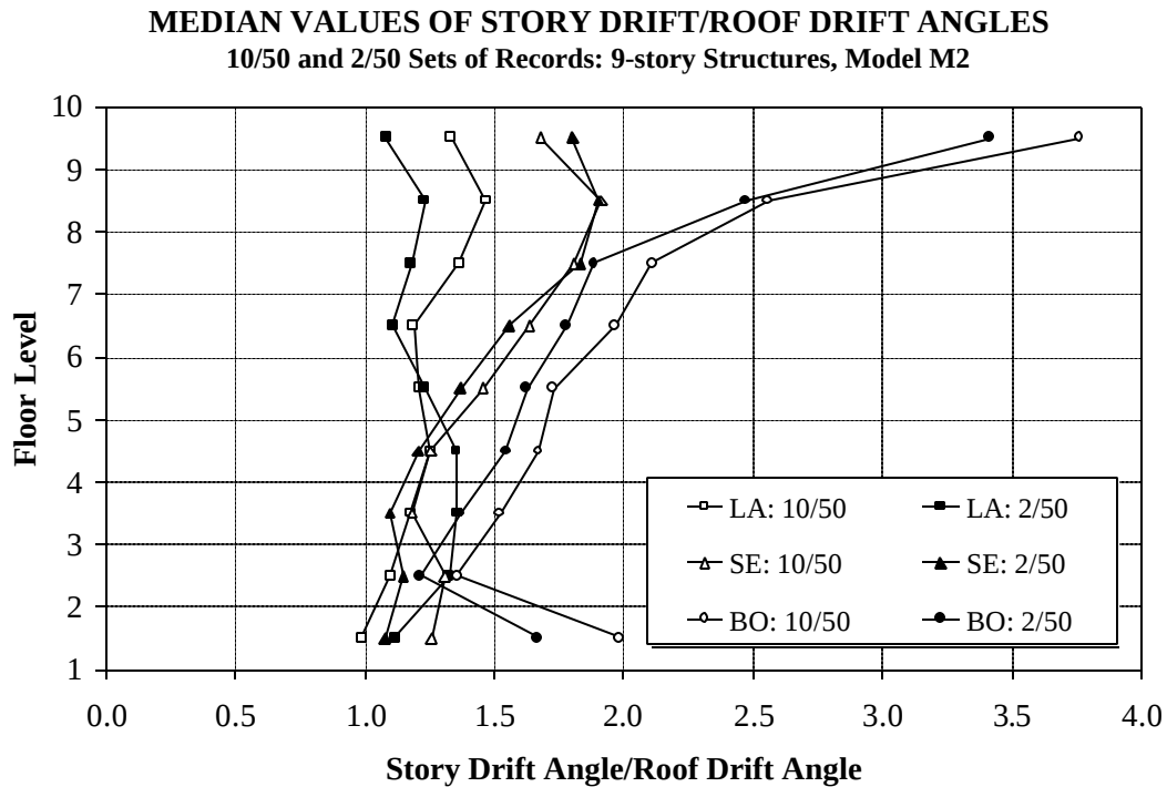
Figure 7.24 Median Values for Ratio of Story Drift Angle to Roof Drift Angle for All 9-story Structures; 10/50 and 2/50 Sets of Records
