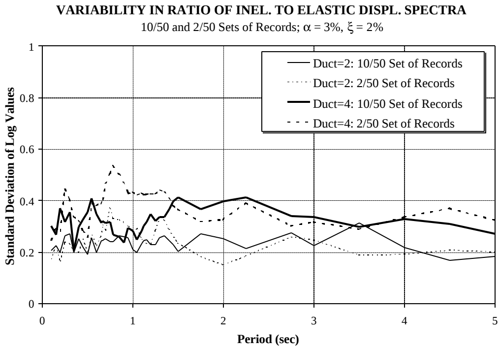
Figure 7.8 Dispersion Associated with Values for Inelastic/Elastic Displacements for SDOF Systems, \alpha = 3\% , \xi = 2\% ; 10/50 and 2/50 Sets of LA Ground Motions
