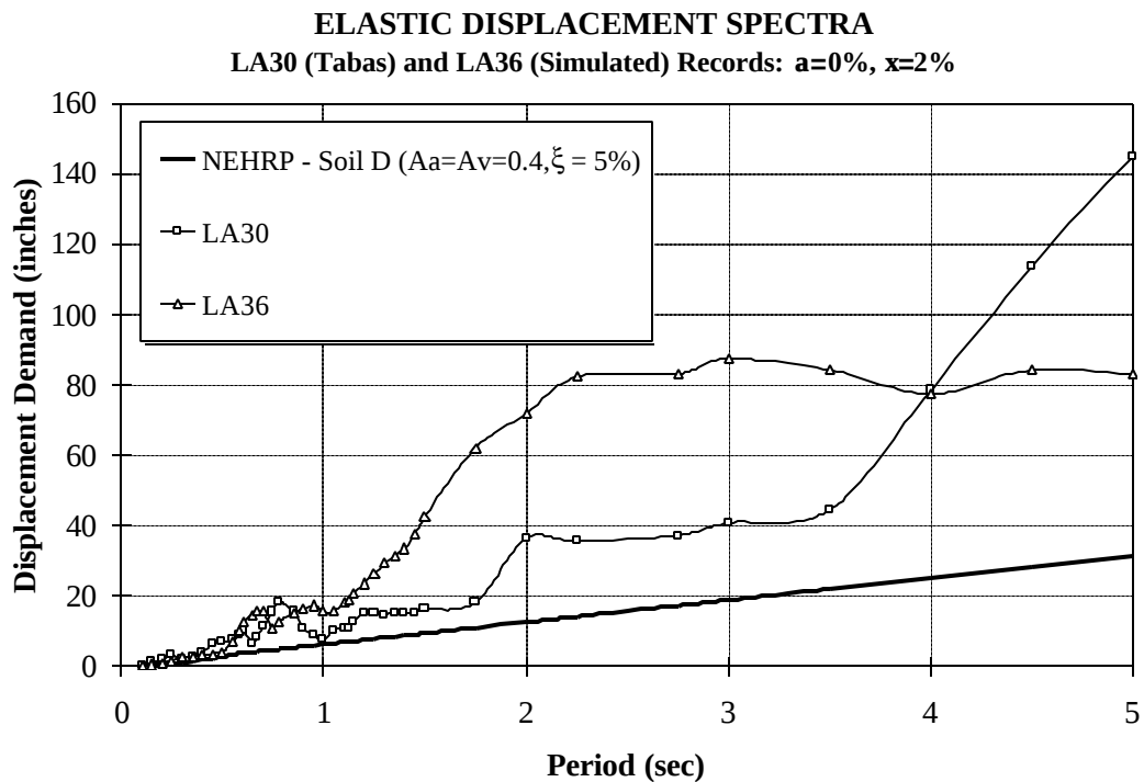
Figure 4.12 Elastic Displacement Spectra for Ground Motions Used for P-delta Study of LA 20-story Structure
