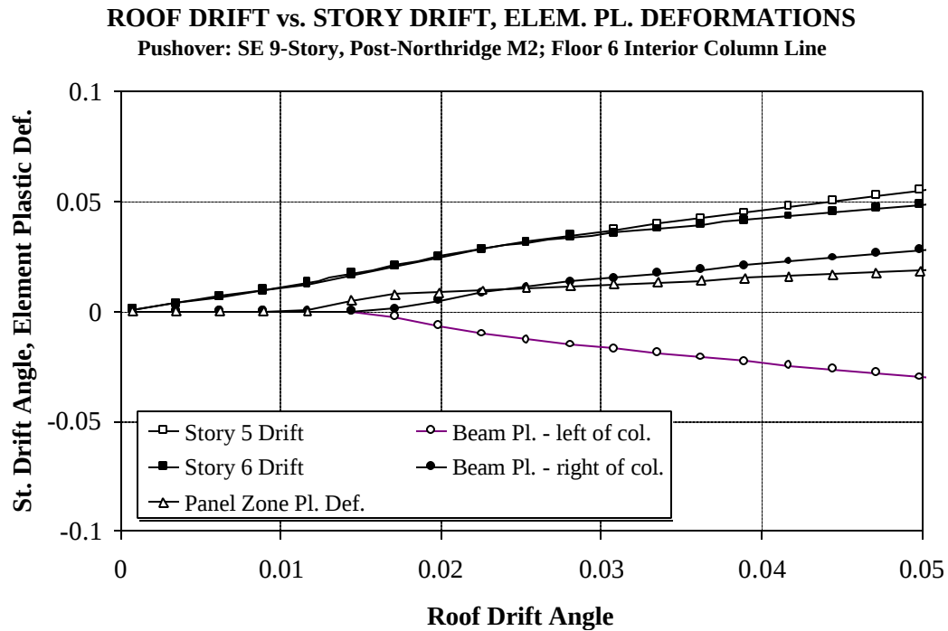
Figure 6.8 Variation of Story and Element Deformation Demands with Increasing Roof Drift Angle for Seattle 9-story Cover-Plated Post-N. Structure; Pushover Analysis
