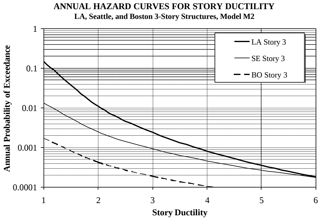
Figure 5.48 Annual Hazard Curves for Story 3 Ductility Demand for LA, Seattle, and Boston 3-story Structures
