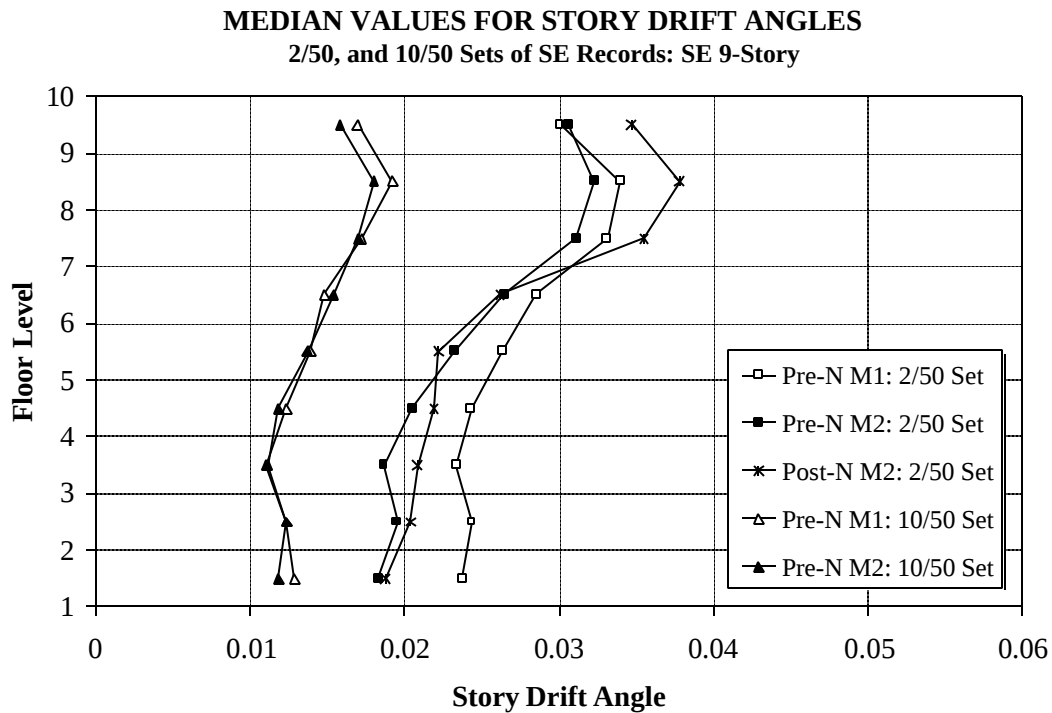
Figure 5.24 Median Values for Story Drift Angle Demands for Seattle 9-story Structures; 10/50 and 2/50 Sets of Ground Motions
