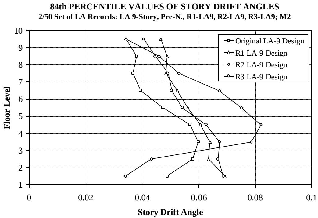
Figure 8.25 84 th Percentile Story Drift Angle Demands for Original and Redesigned LA 9-story Structures; 2/50 Set of Ground Motions
