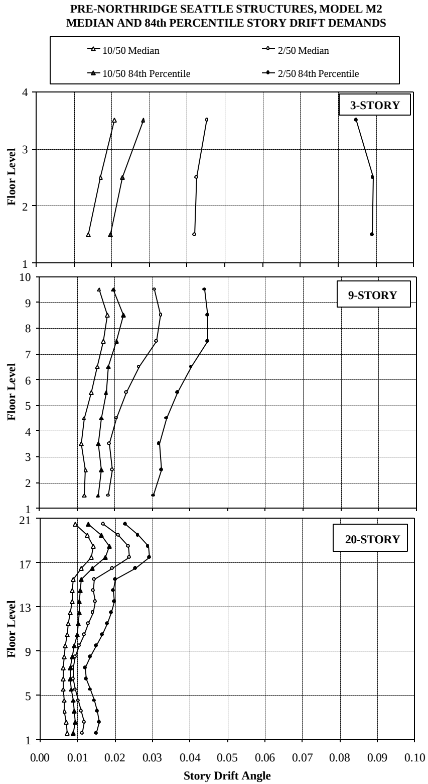
Figure 5.32 Median and 84 th Percentile Story Drift Angle Demands for Seattle Structures, Model M2; 10/50 and 2/50 Sets of Ground Motions
