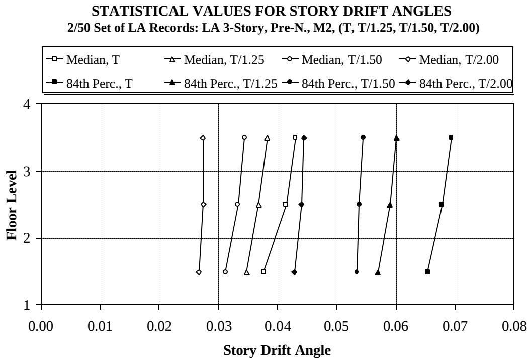
Figure 8.18 Sensitivity of Story Drift Angle Demands to Period of Structure, LA 3-story Structure; 2/50 Set of Ground Motions
