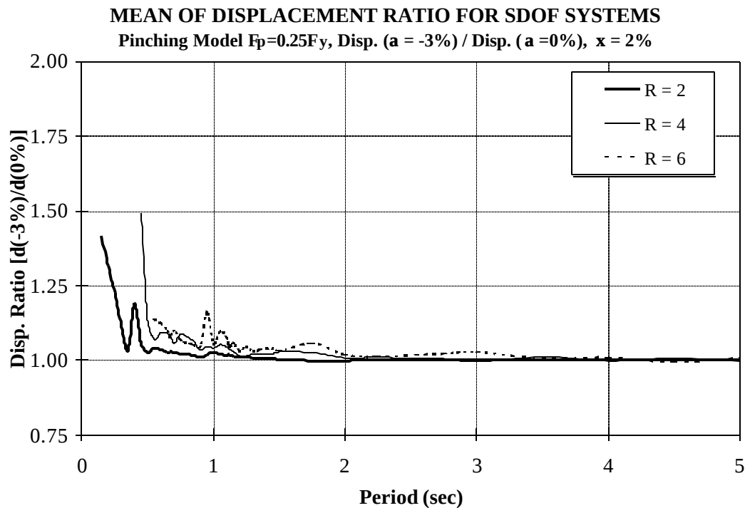
Figure 8.8 Effect of P-delta on Displacement Demands for SDOF Systems with Stiffness Degradation (75% Pinching); 2/50 Set of Ground Motions
