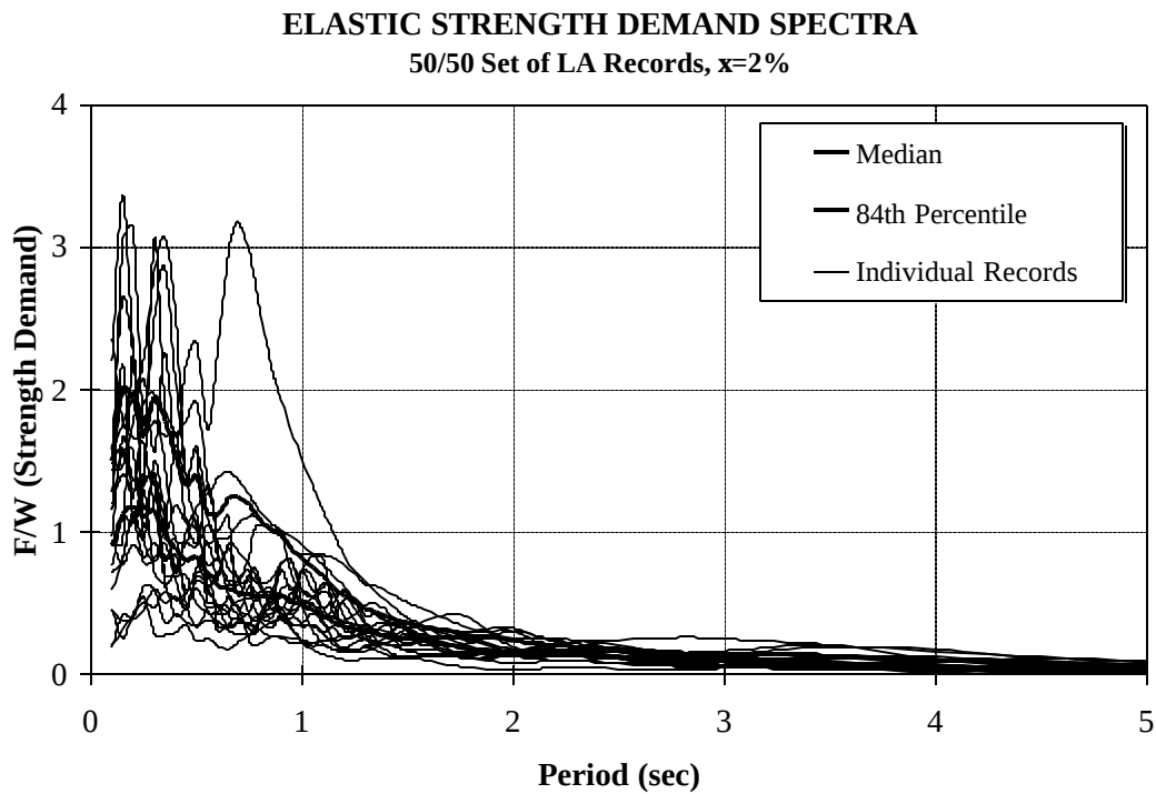
Figure A.1 Elastic Strength Demand (Acceleration) Spectra, 50/50 Set of LA Ground Motions
