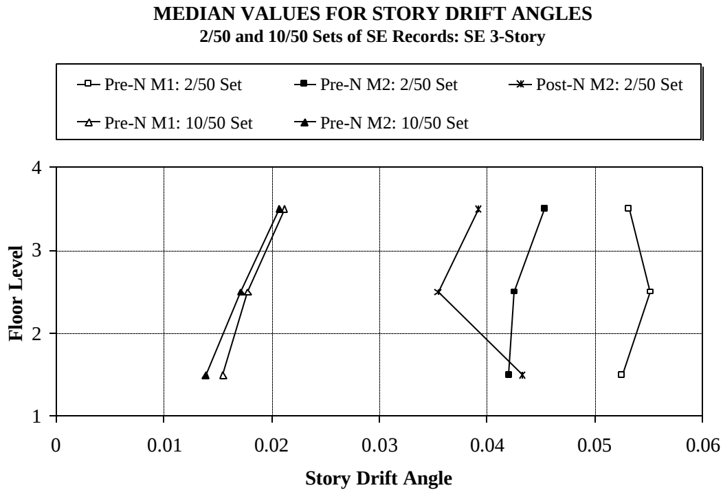
Figure 5.23 Median Values for Story Drift Angle Demands for Seattle 3-story Structures; 10/50 and 2/50 Sets of Ground Motions
