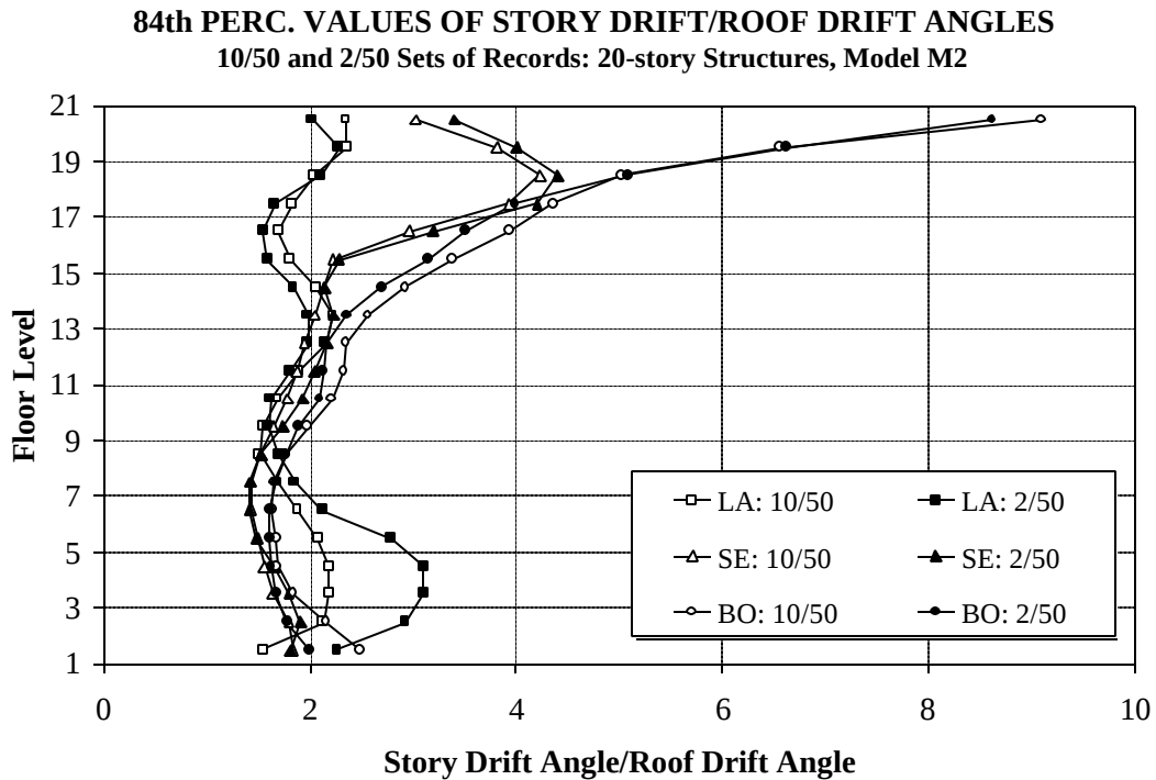
Figure 7.26 84 th Percentile Values for Ratio of Story Drift Angle to Roof Drift Angle for LA, Seattle, and Boston 20-story Structures; 10/50 and 2/50 Sets of Records
