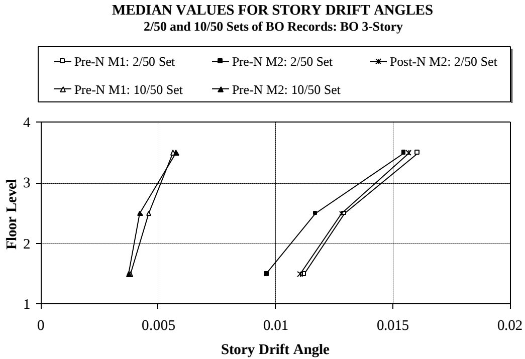
Figure 5.27 Median Values of Story Drift Angle Demands for Boston 3-story Structures; 10/50 and 2/50 Sets of Ground Motions
