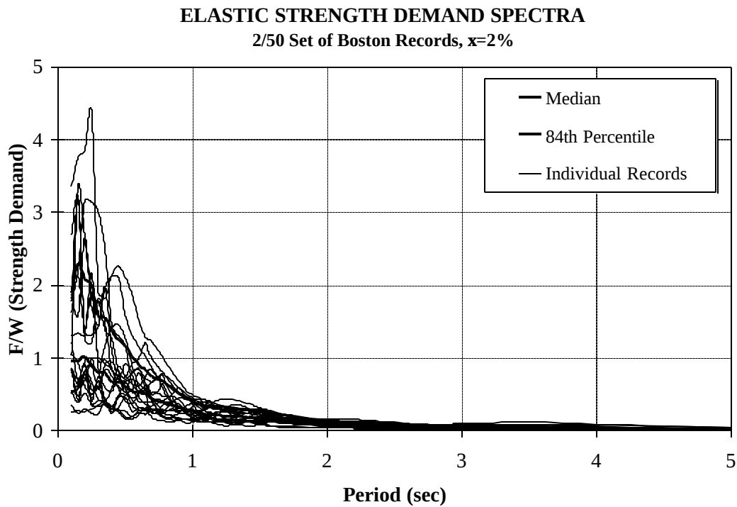
Figure A.13 Elastic Strength Demand (Acceleration) Spectra, 2/50 Set of Boston Ground Motions
