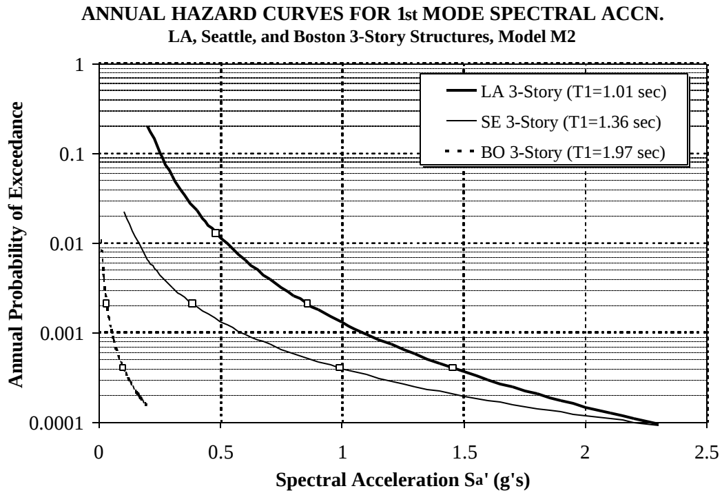
Figure 5.45 Annual Hazard Curves for 1 st Mode Spectral Acceleration for LA, Seattle, and Boston 3-story Structures
