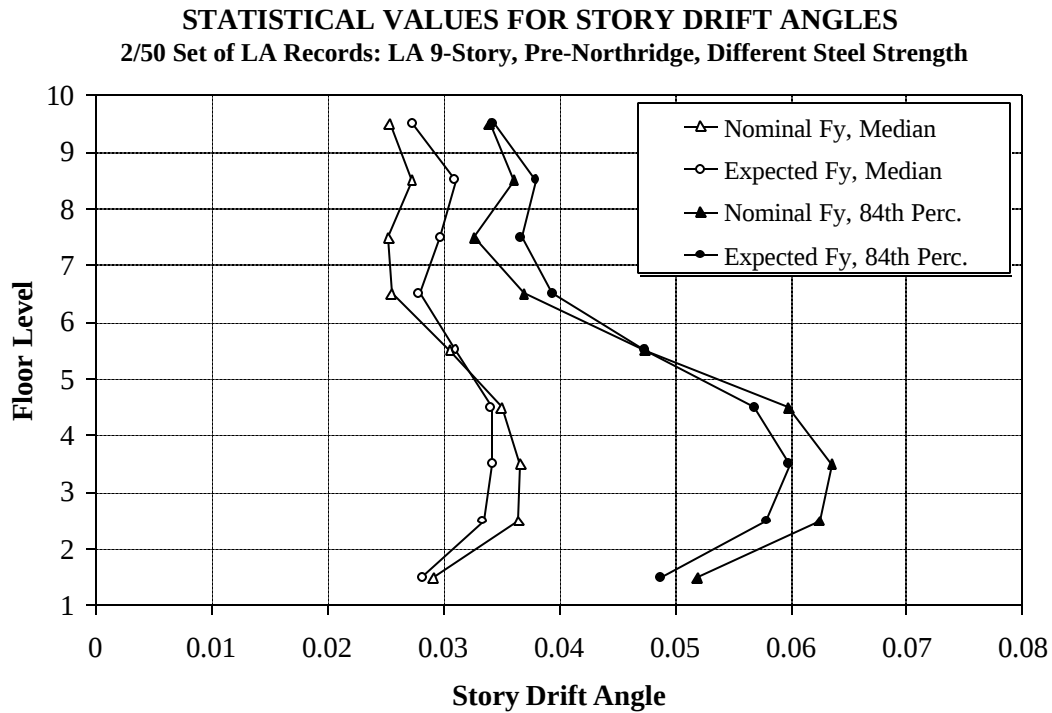
Figure 6.11 Story Drift Angle Demands for LA 9-story Structure with Expected and Nominal Strength Properties; 2/50 Set of Ground Motions
