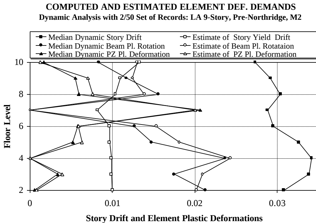
Figure 7.37 Comparison of Element Plastic Deformation Demands From Simplified Procedure and Inelastic Analysis, LA 9-story Structure; 2/50 Set of Records
