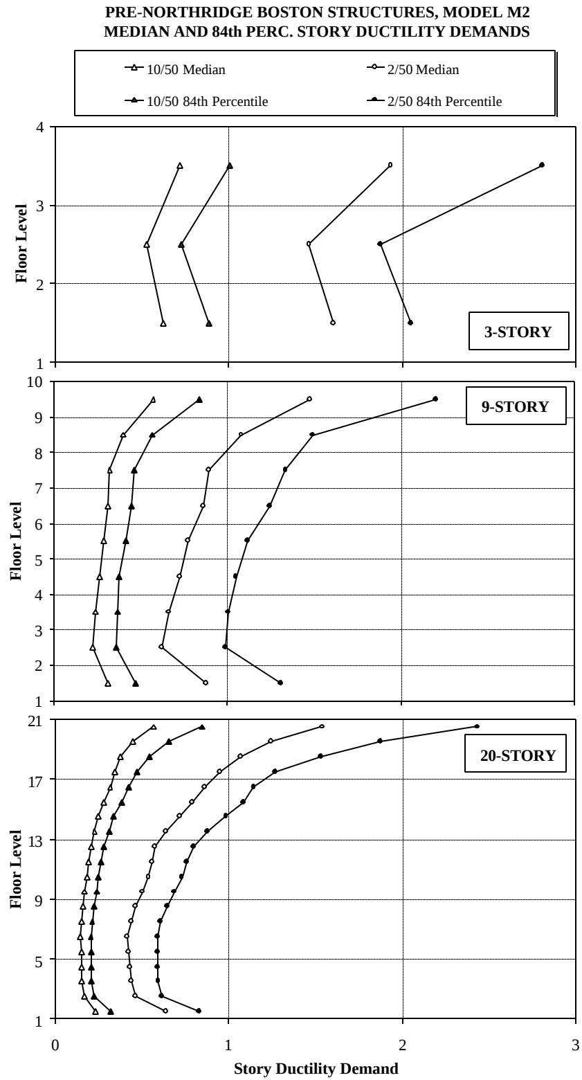
Figure 5.36 Median and 84 th Percentile Story Ductility Demands for Boston Structures, Model M2; 10/50 and 2/50 Sets of Ground Motions
