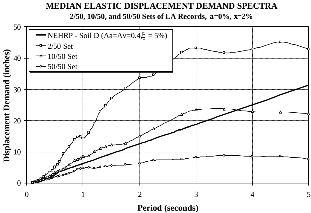
Figure 5.15 Median Values of Elastic Spectral Displacement Demands for LA 50/50, 10/50, and 2/50 Sets of Ground Motions
