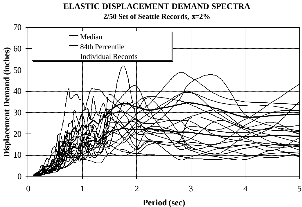
Figure A.10 Elastic Displacement Demand Spectra, 2/50 Set of Seattle Ground Motions
