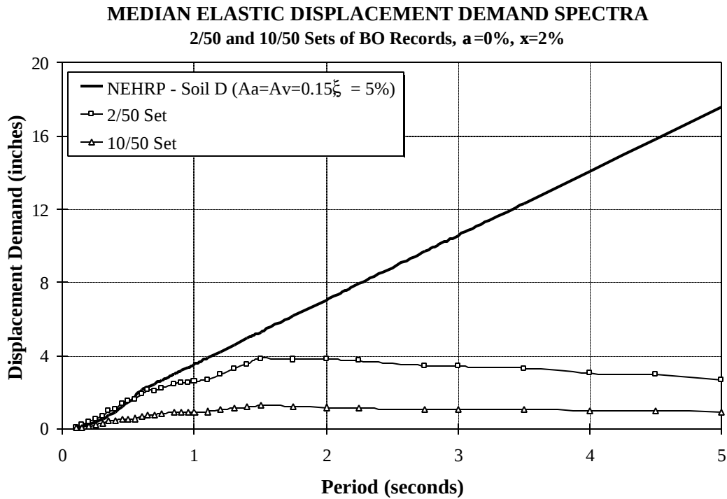
Figure 5.17 Median Values of Elastic Spectral Displacement Demands for Boston 10/50 and 2/50 Sets of Ground Motions
