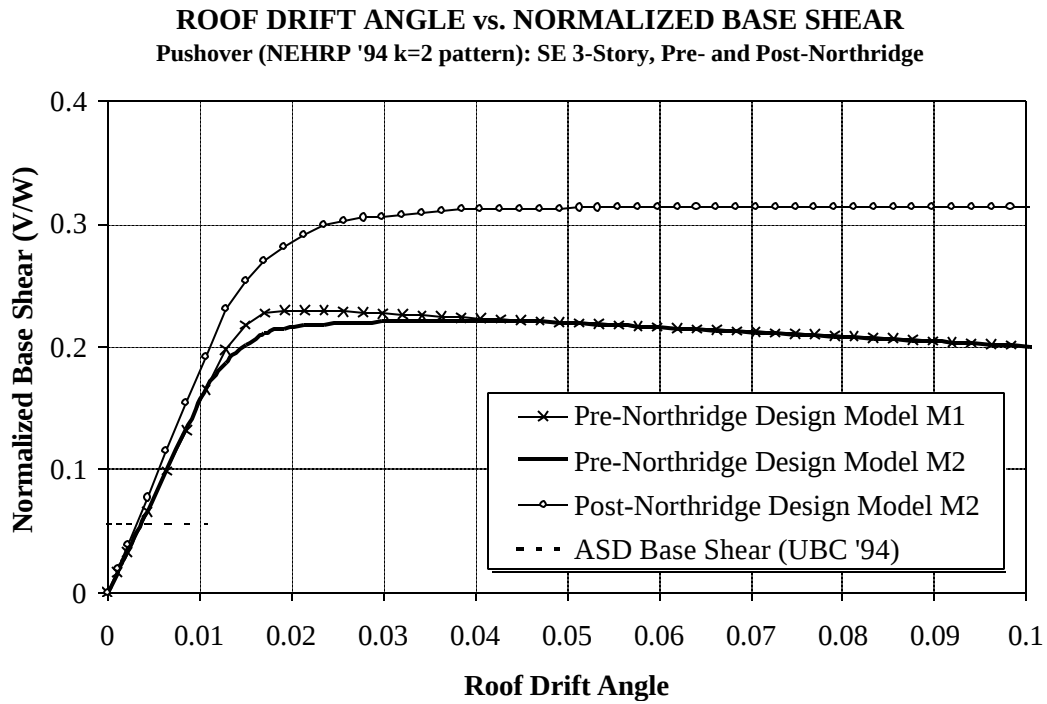
Figure 5.5 Global Pushover Curves for Seattle 3-story Structures
