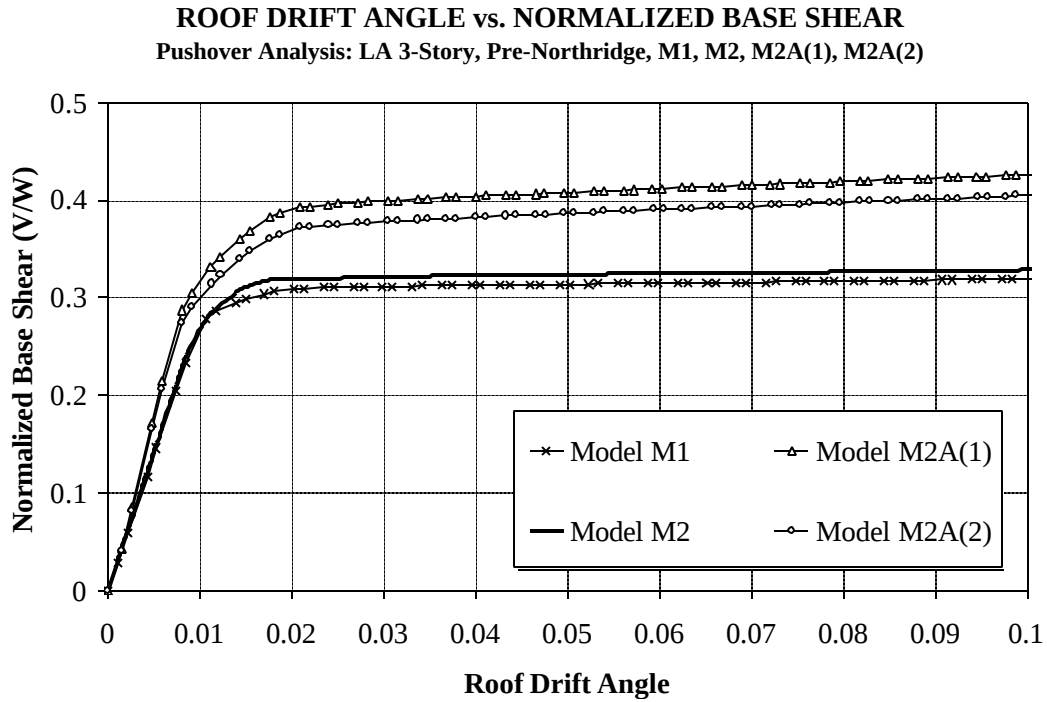
Figure 3.10 Global Pushover Curves for LA 3-story Structure, Different Models
