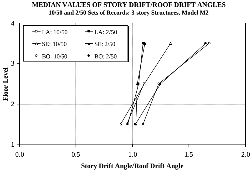
Figure 7.23 Median Values for Ratio of Story Drift Angle to Roof Drift Angle for All 3-story Structures; 10/50 and 2/50 Sets of Records
