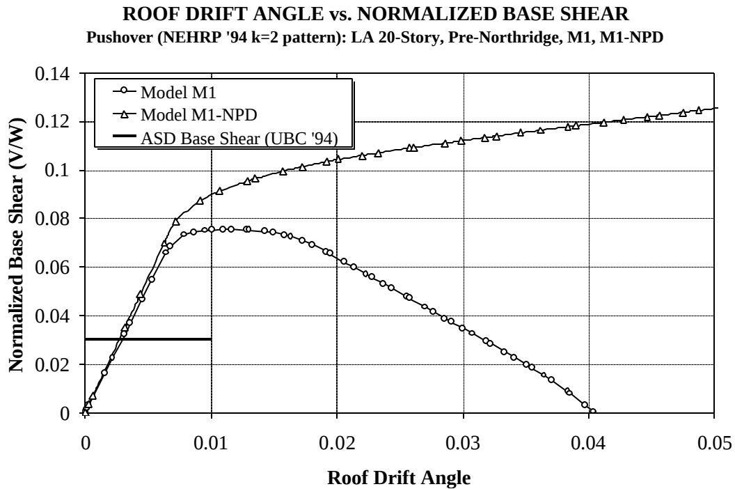
Figure 4.5 Global Pushover Curves for Model M1 of LA20-story Structure, without and with P-delta
