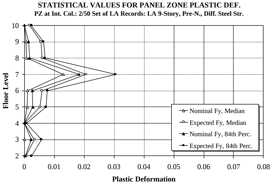
Figure 6.15 Panel Zone (@ Interior Col.) Plastic Deformation Demands for LA 9-story Structure with Expected and Nominal Strength Properties; 2/50 Set of Ground Motions
