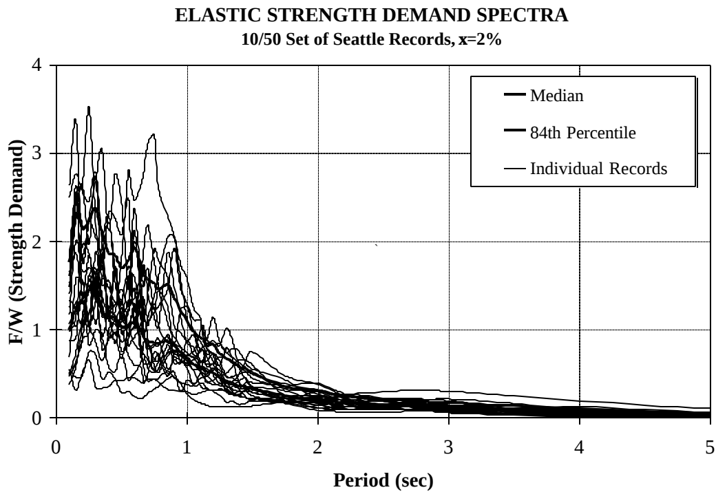
Figure A.7 Elastic Strength Demand (Acceleration) Spectra, 10/50 Set of Seattle Ground Motions
