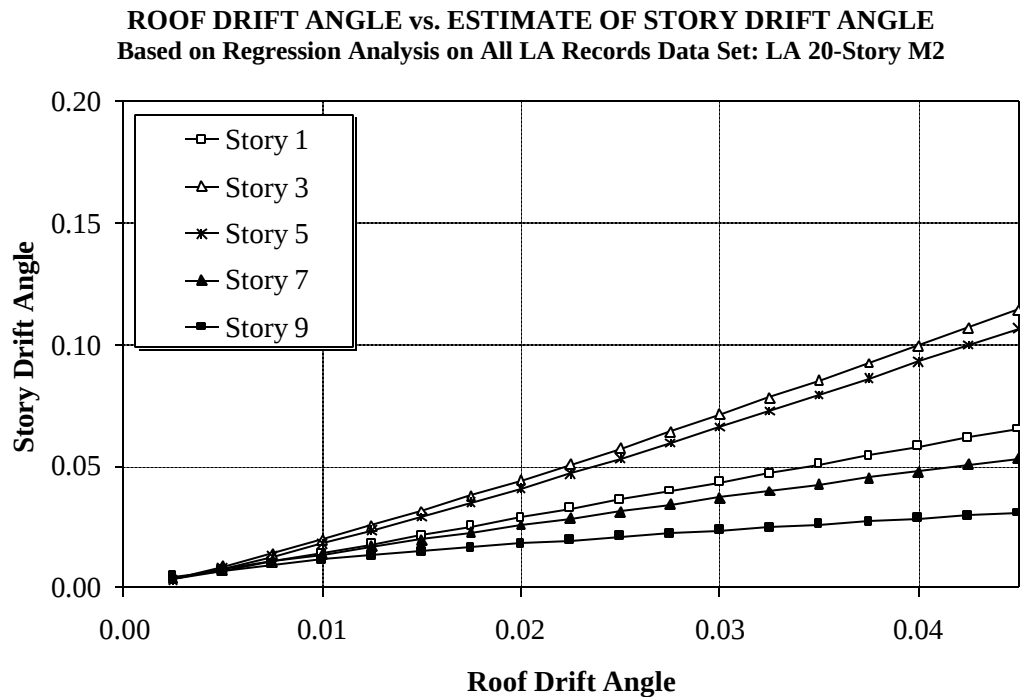
Figure 7.32 Relationship Between Story Drift Angles and Roof Drift Angle for LA 20-story Structure, Based on Regression Analysis; All LA Records
