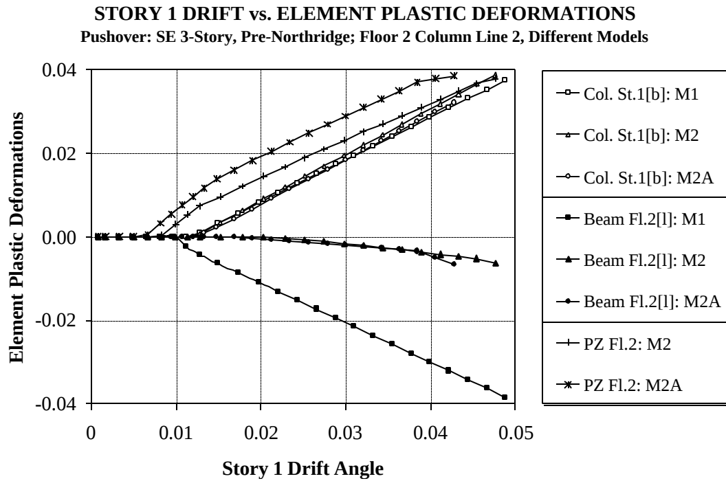
Figure 3.16 Element Plastic Deformations Versus Story 1 Drift Angle, Seattle 3-story Structure, Different models; Pushover Analysis
