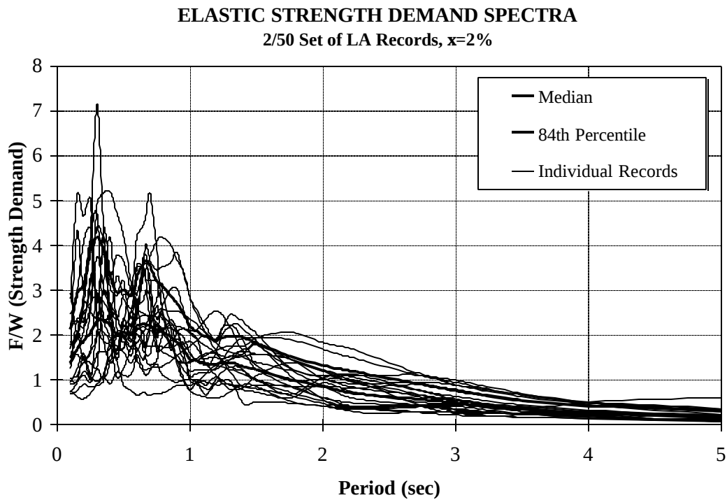
Figure A.5 Elastic Strength Demand (Acceleration) Spectra, 2/50 Set of LA Ground Motions
