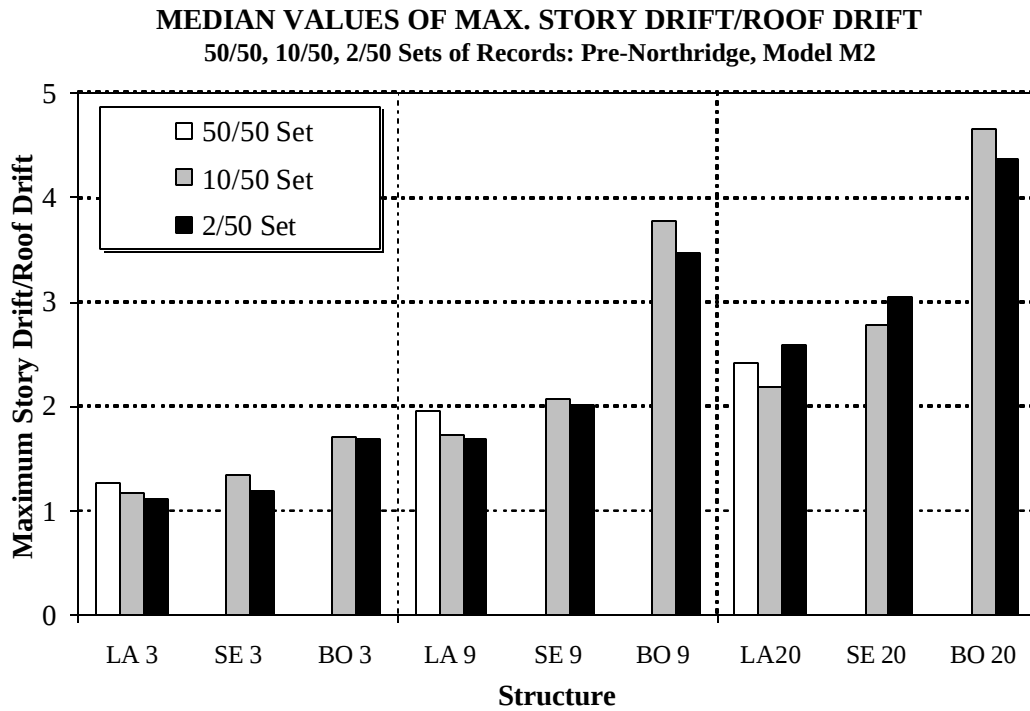
Figure 7.21 Median Values for Ratio of Max. Story Drift to Roof Drift for All Structures; All Sets of Records
