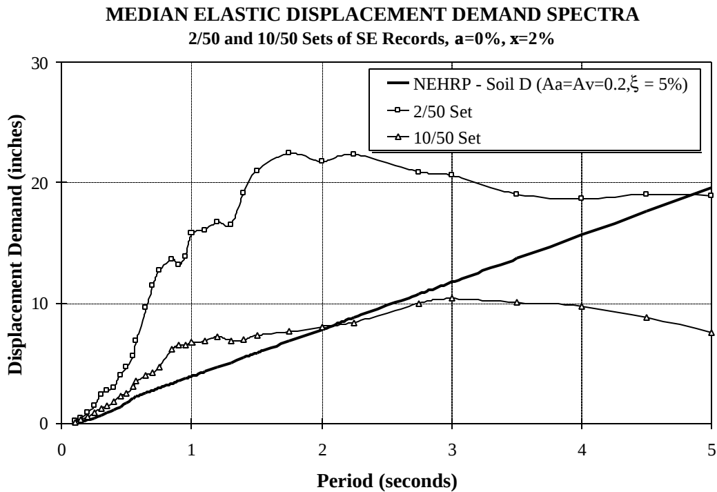
Figure 5.16 Median Values of Elastic Spectral Displacement Demands for Seattle 10/50 and 2/50 Sets of Ground Motions
