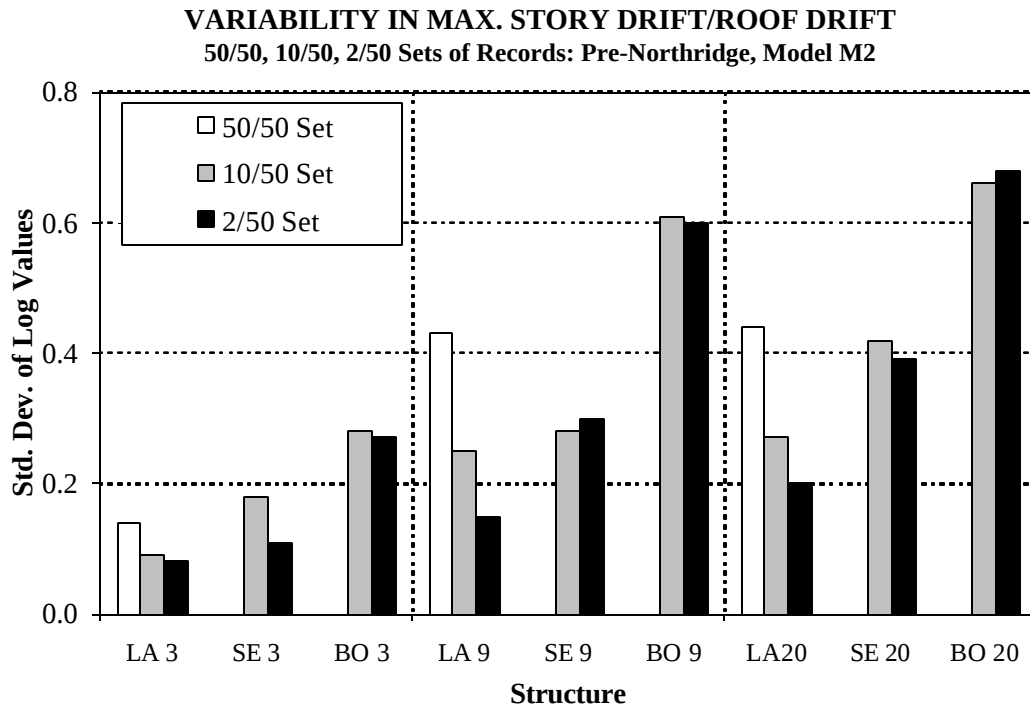
Figure 7.22 Dispersion Associated with Ratio of Max. Story Drift to Roof Drift for All Structures; All Sets of Records
