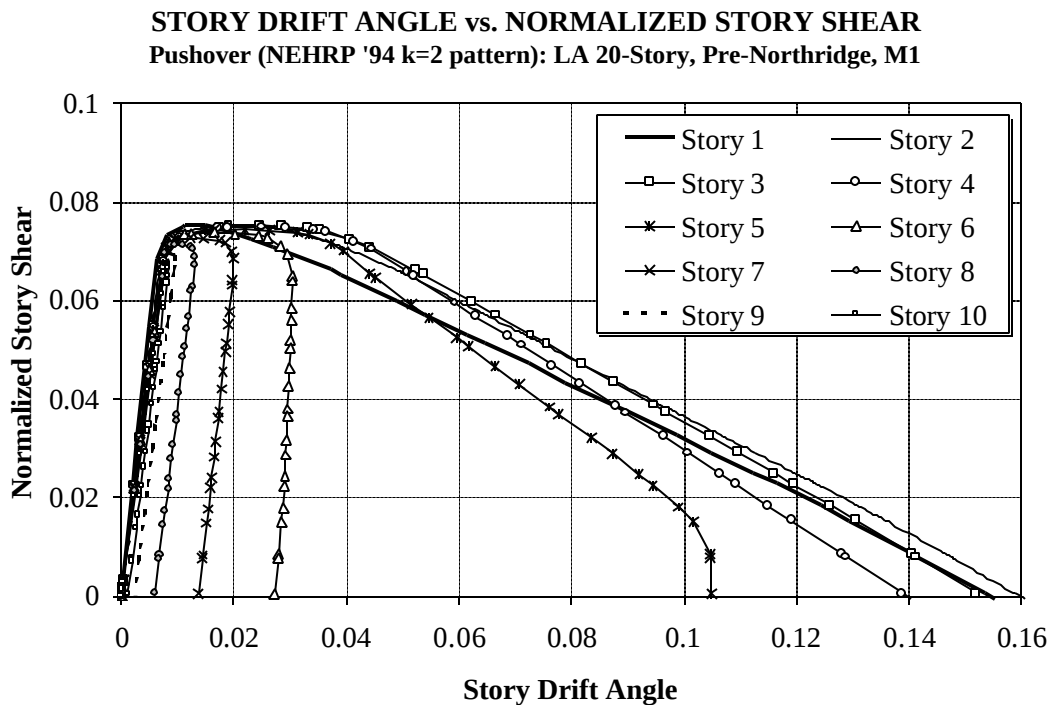
Figure 4.6 Story Shear versus Story Drift Diagrams for Model M1 of LA 20-story Structure; Pushover Analysis
