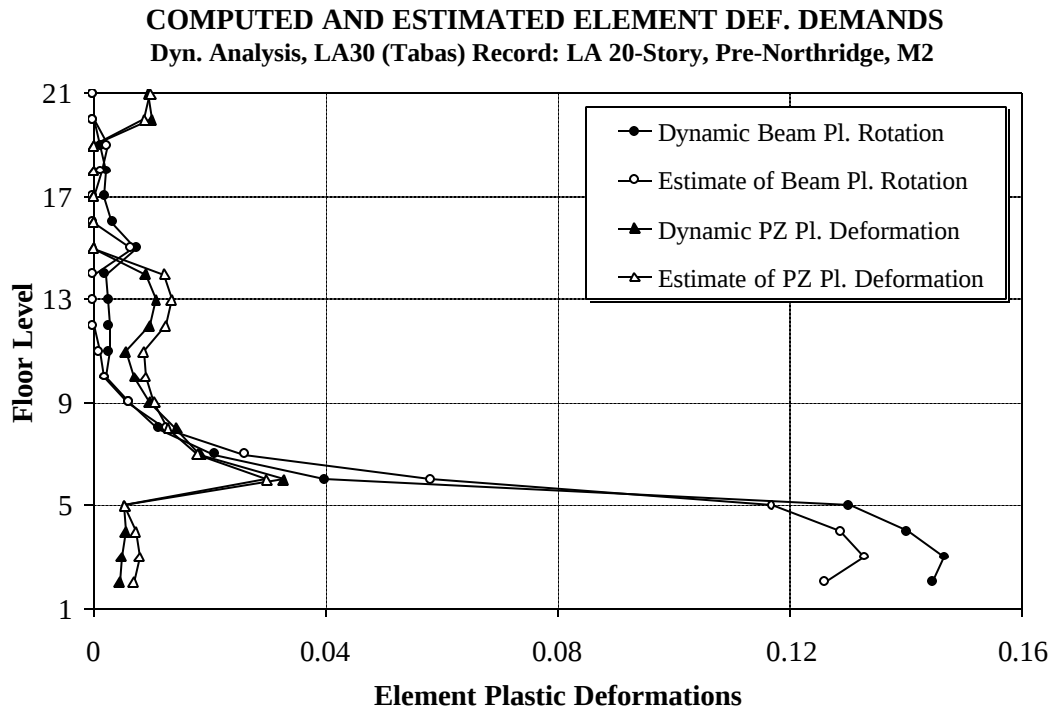
Figure 7.40 Comparison of Element Plastic Deformation Demands From Simplified Procedure and Inelastic Analysis, LA 20-story Structure; LA30 (Tabas) Record
