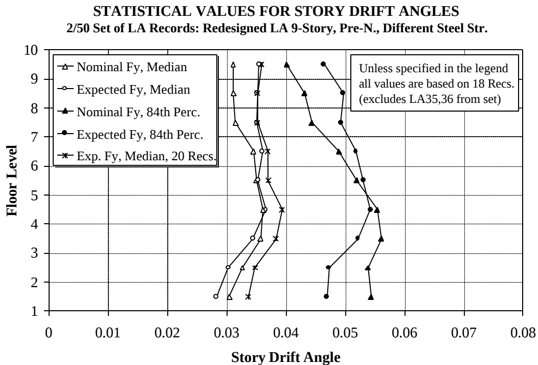
Figure 6.12 Story Drift Angle Demands for Redesigned LA 9-story Structure with Expected and Nominal Strength Properties; 2/50 Set of Ground Motions
