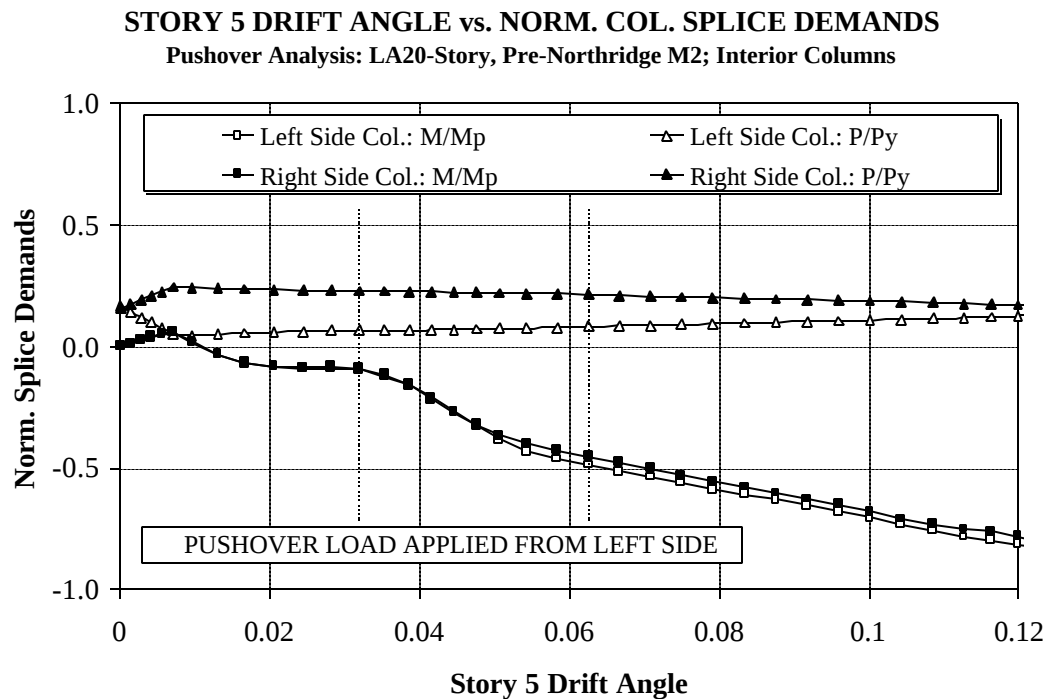
Figure 6.32 Variation of Normalized Force Demands for Interior Column Splices in Story 5 with Increasing Story 5 Drift; LA 20-story; Pushover Analysis
