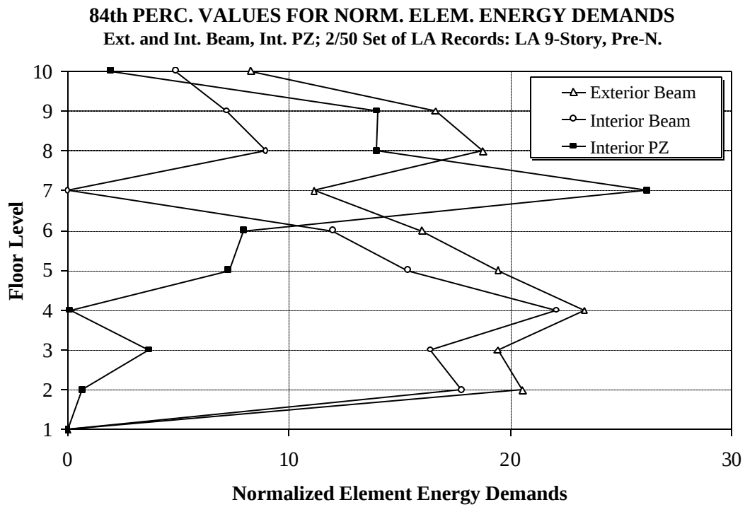
Figure 6.41 84 th Percentile for Normalized Element Energy Dissipation Demands, LA 9-story Structure; 2/50 Set of Ground Motions
