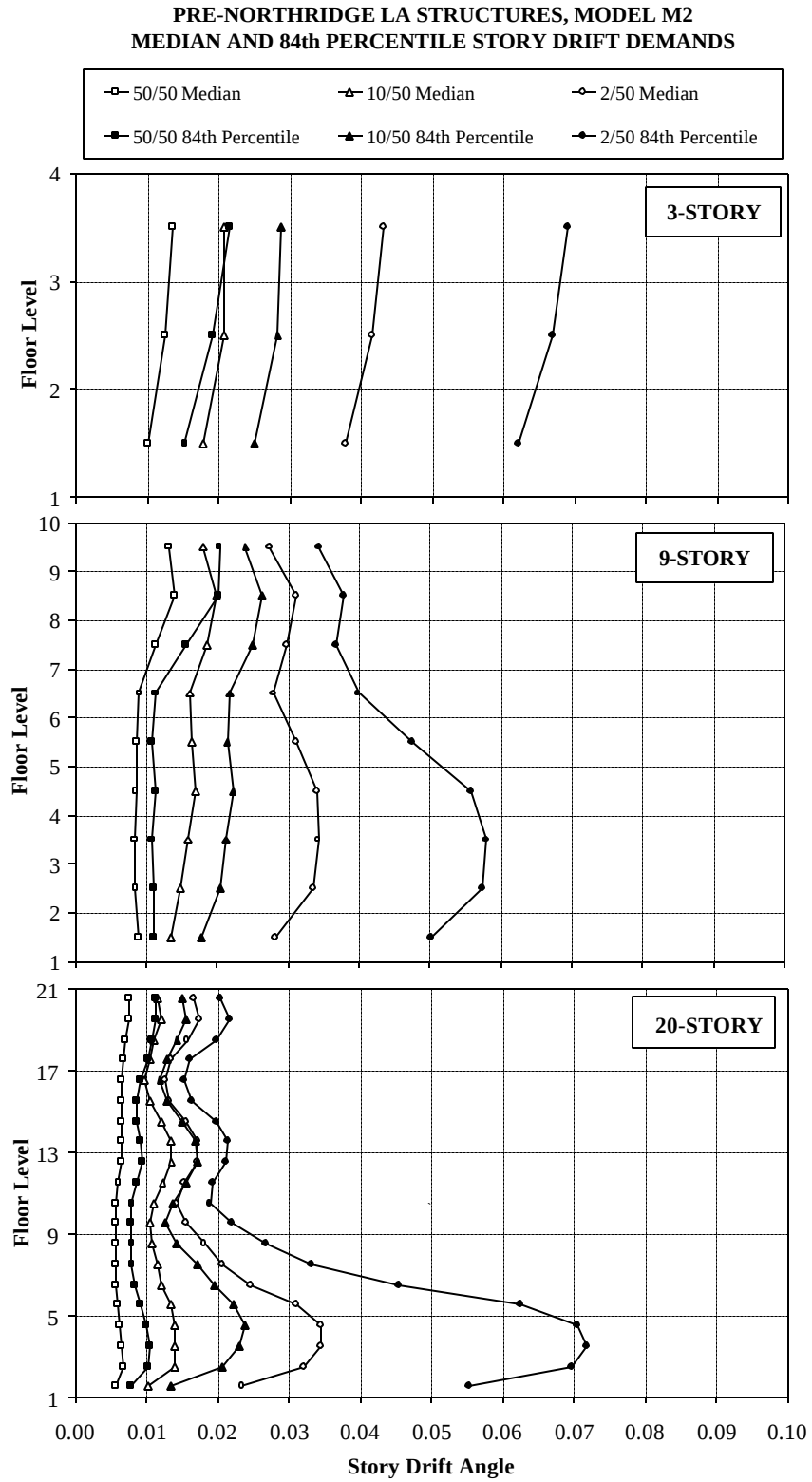
Figure 5.31 Median and 84 th Percentile Story Drift Angle Demands for LA Structures, Model M2; 50/50, 10/50, and 2/50 Sets of Ground Motions
