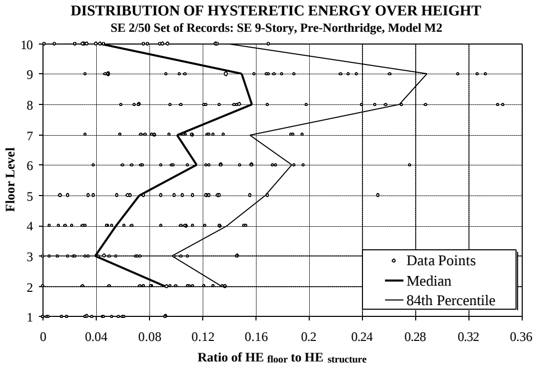
Figure 5.61 Distribution of Hysteretic Energy Demands Over the Height of 9-story Seattle Structure; 2/50 Set of Ground Motions
