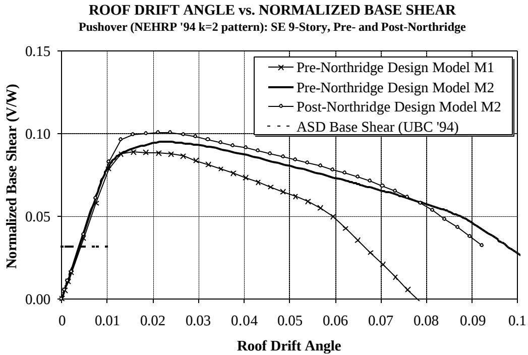
Figure 5.6 Global Pushover Curves for Seattle 9-story Structures
