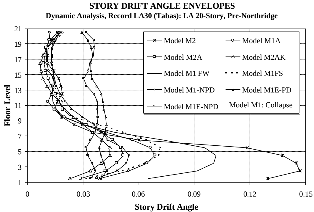
Figure 4.17 Maximum Story Drift Angles for Various Models of LA 20-story Structure; LA30 (Tabas) Ground Motion
