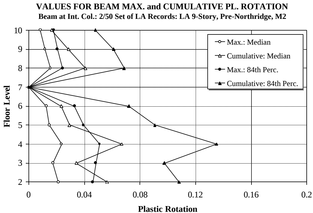
Figure 6.34 Statistical Values for Interior Beam End Maximum and Cumulative Plastic Rotation Demands, LA 9-story Structure; 2/50 Set of Ground Motions
