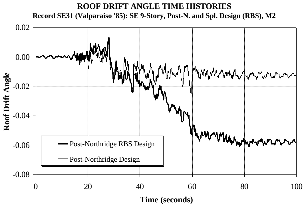
Figure 6.18 Roof Drift Time History of Response of Seattle 9-story Cover-Plated Post-N. and RBS Design; SE31 Ground Motion
