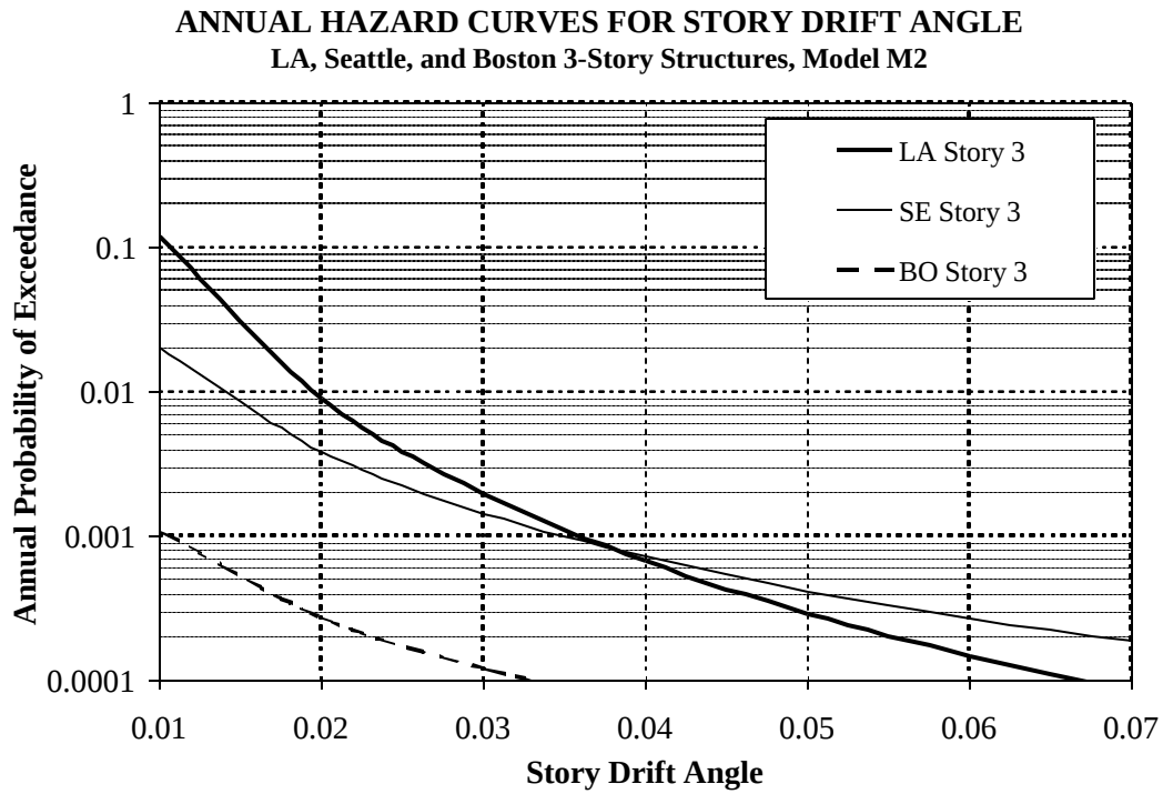
Figure 5.47 Annual Hazard Curves for Story 3 Drift Angle Demand for LA, Seattle, and Boston 3-story Structures
