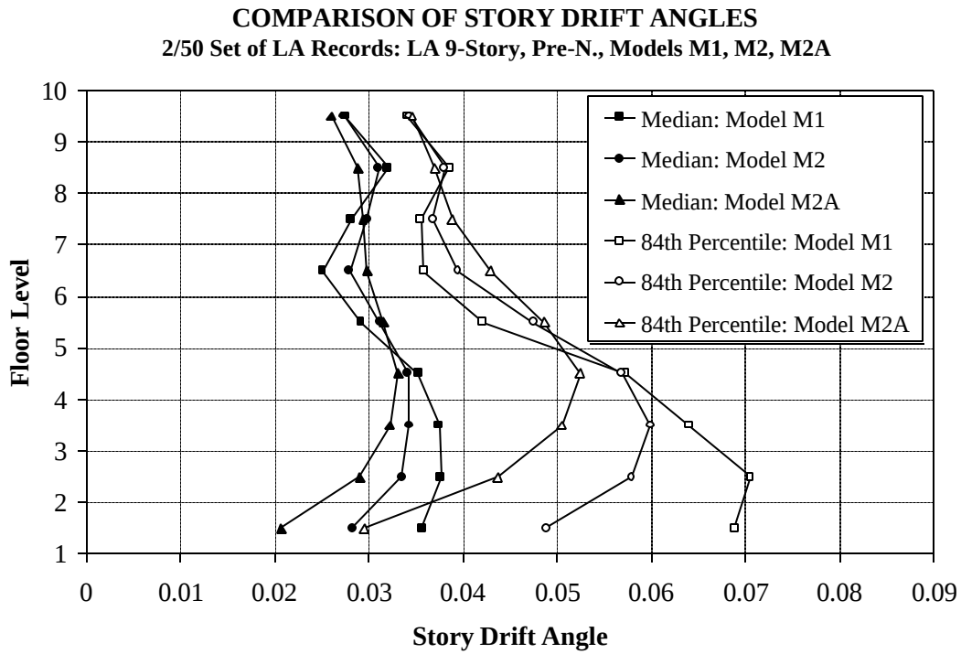
Figure 3.20 Median and 84 th Percentile Values of Story Drift Demands for LA 9-story Structure, Different Models; 2/50 Set of Ground Motions
