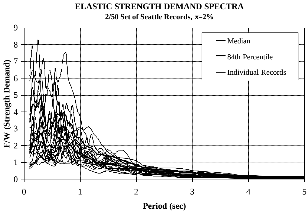
Figure A.9 Elastic Strength Demand (Acceleration) Spectra, 2/50 Set of Seattle Ground Motions
