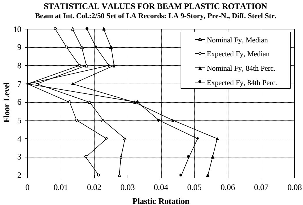
Figure 6.14 Beam (@ Interior Col.) Plastic Rotation Demands for LA 9-story Structure with Expected and Nominal Strength Properties; 2/50 Set of Ground Motions
