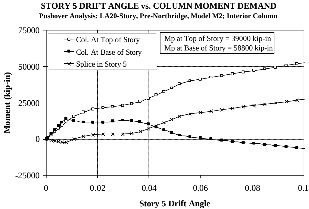
Figure 6.23 Variation of Bending Moment at Top and Base of Story 5 Interior Column with Increasing Story Drift, LA 20-story; Pushover Analysis
