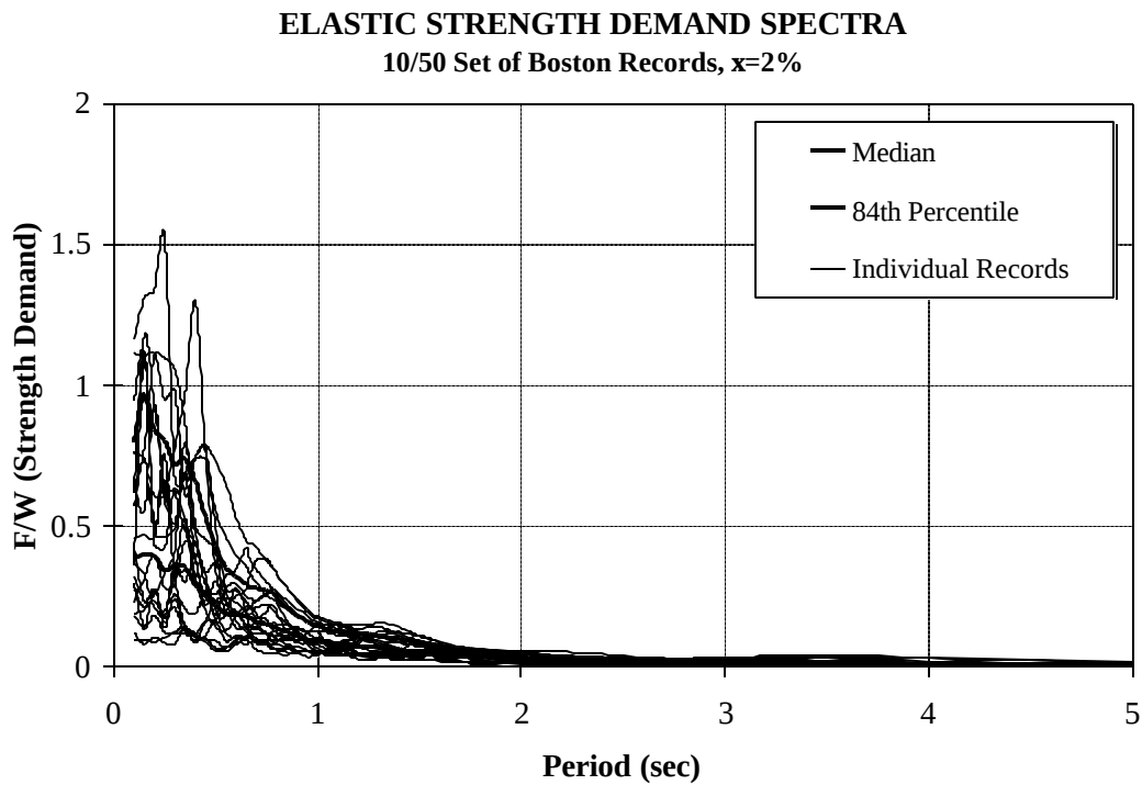
Figure A.11 Elastic Strength Demand (Acceleration) Spectra, 10/50 Set of Boston Ground Motions
