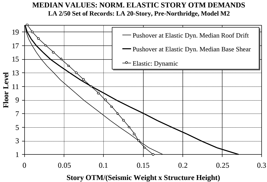
Figure 5.57. Median Story OTM Demands Under 2/50 Sets of Ground Motions, Compared to Demands From Pushover Analysis, for Elastic LA 20-story Structure
