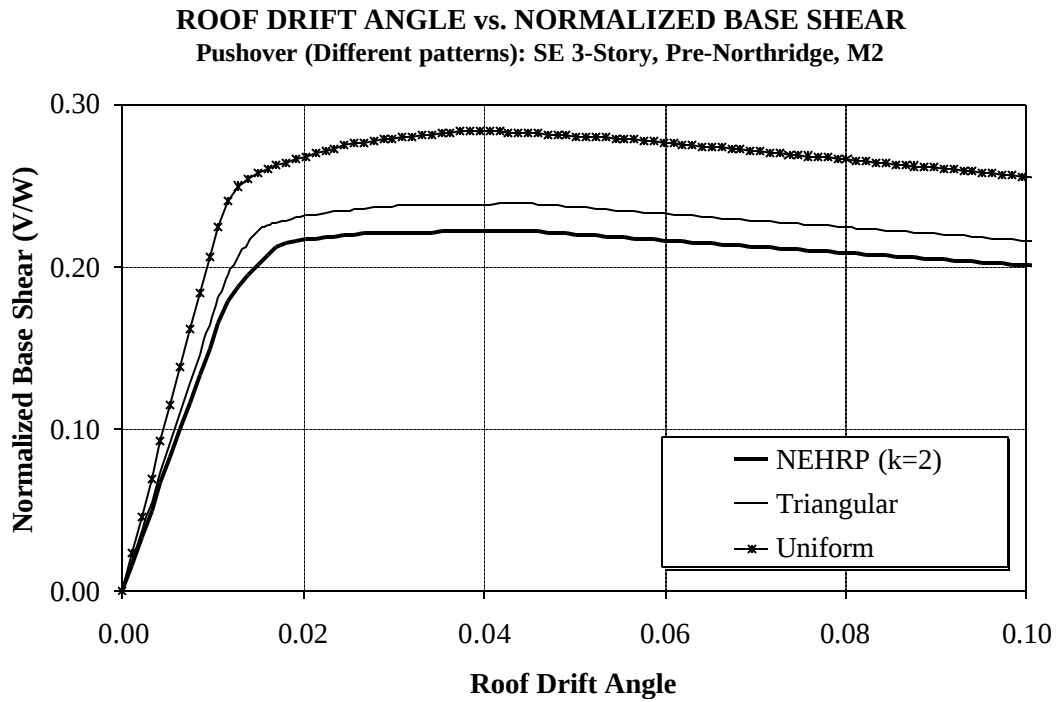
Figure 7.20 Effect of Load Pattern on Global (Roof) Pushover Response for Seattle 3-story Structure, Model M2
