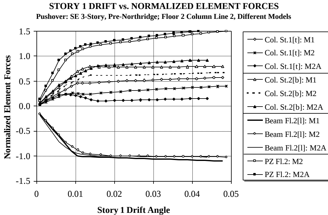
Figure 3.17 Element Force Demands Versus Story 1 Drift Angle, Seattle 3-story Structure, Different Models; Pushover Analysis
