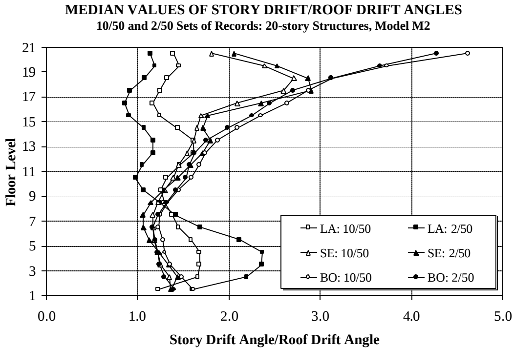
Figure 7.25 Median Values for Ratio of Story Drift Angle to Roof Drift Angle for All 20-story Structures; 10/50 and 2/50 Sets of Records
