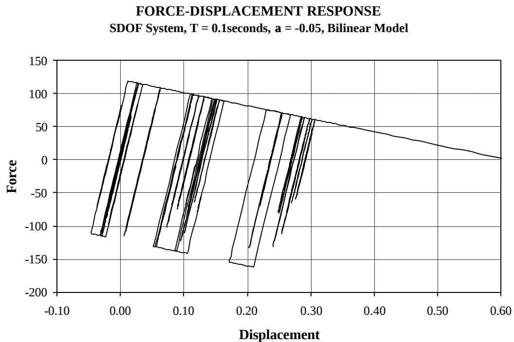
Figure 4.2 Dynamic Lateral Force - Displacement Response of SDOF System with T = 0.1 and a = -0.05 .
