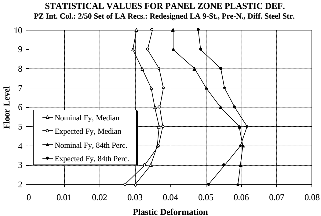
Figure 6.16 Panel Zone (@ Interior Col.) Plastic Deformation Demands for Redesigned LA 9-story Str., with Exp. and Nominal Strength Properties; 2/50 Set of Ground Motions
